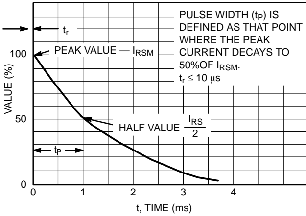
Figure 1. 10 × 1000 μs Pulse Waveform
