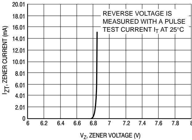
Figure 3. Zener Voltage vs. Zener Current
