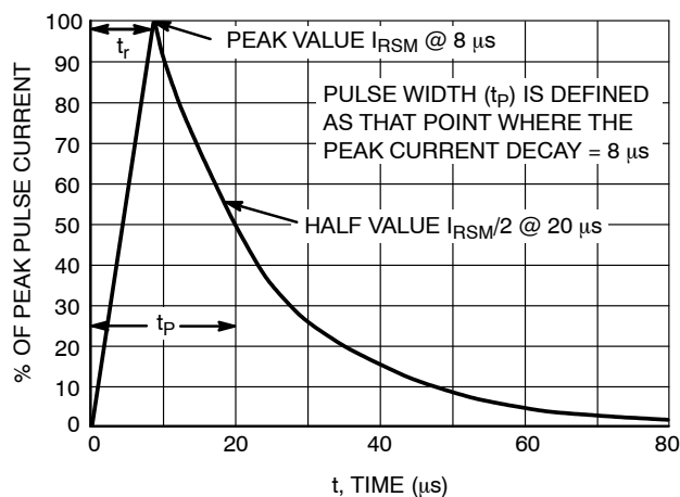
Figure 9. 8 \times 20 \mu\text{s} Pulse Waveform
