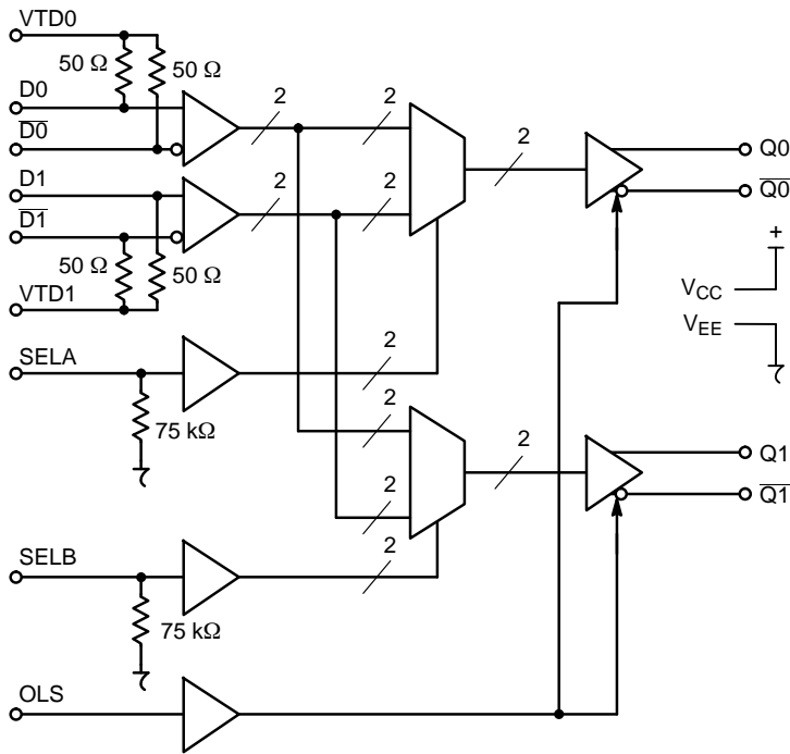
Figure 2. Logic/Block Diagram
