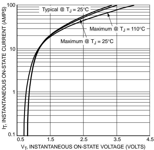
Figure 7. Typical On-State Characteristics
