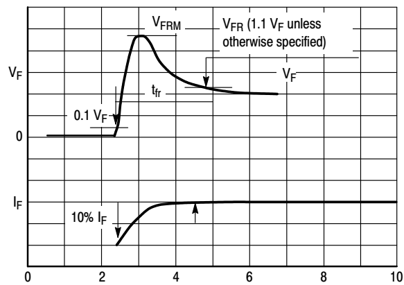
Figure 27. t_{fr} Measurements
