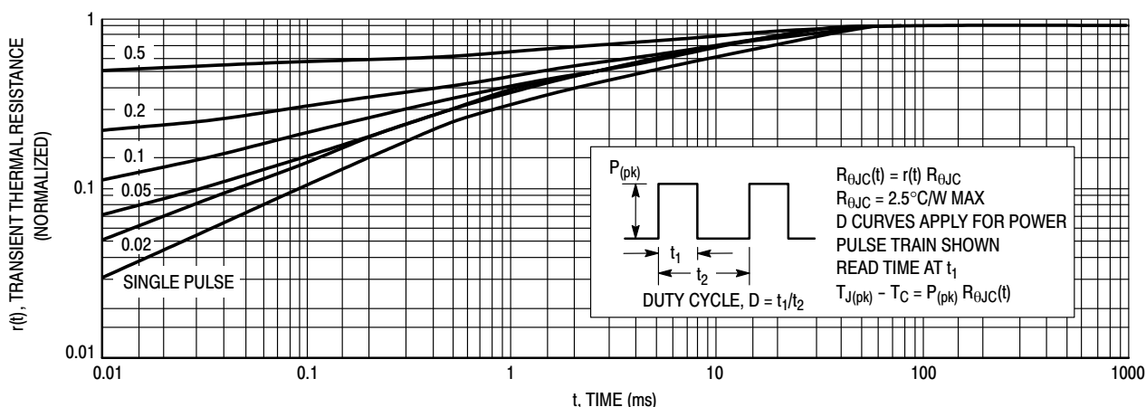
Figure 31. Typical Thermal Response ( Z_{\theta JC}(t) ) for BUL45D2
