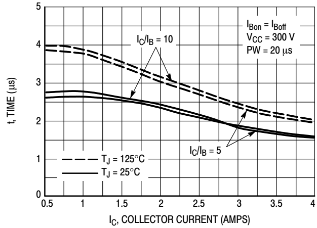
Figure 14. Resistive Switch Time, t_{off}
