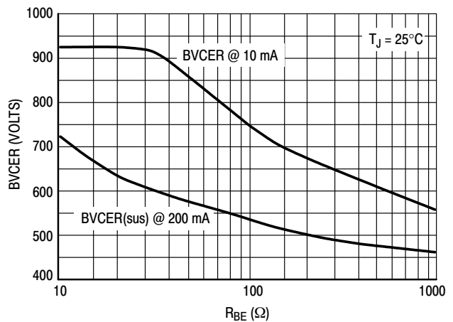
Figure 12. BVCEr = f(ICER)
