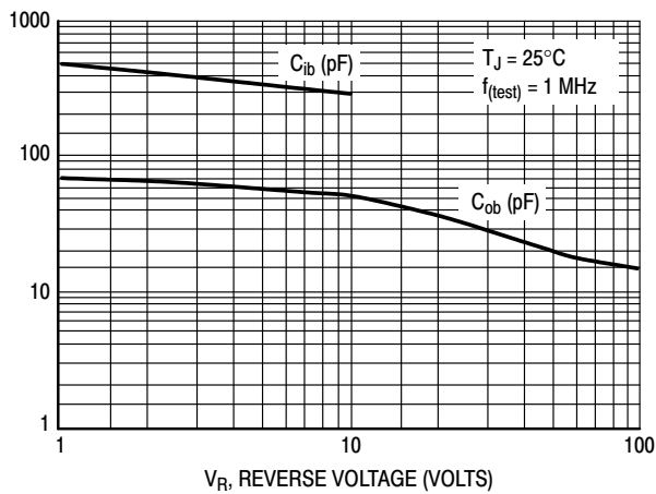
Figure 11. Capacitance
