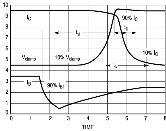
Figure 26. Inductive Switching Measurements
