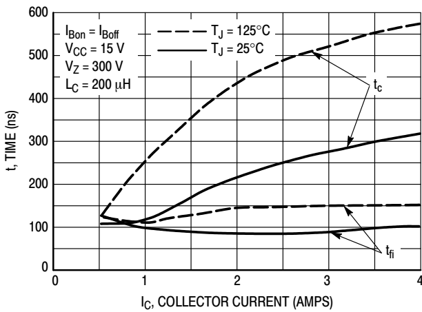
Figure 17. Inductive Switching, t_c & t_{fi} @ I_C/I_B = 5
