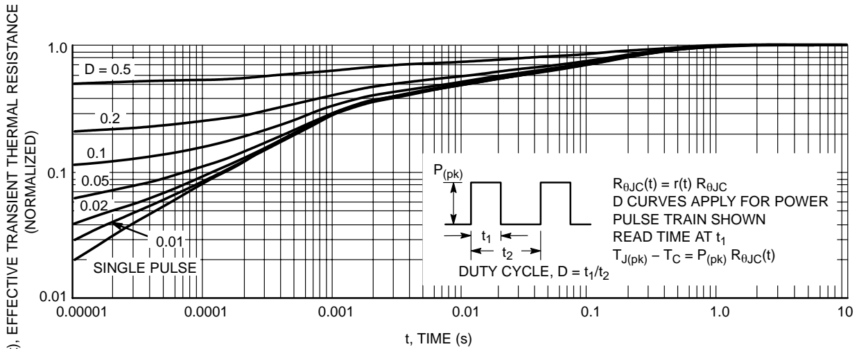
Figure 13. Thermal Response
