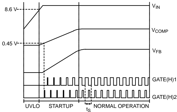
Figure 4. Idealized Waveforms
