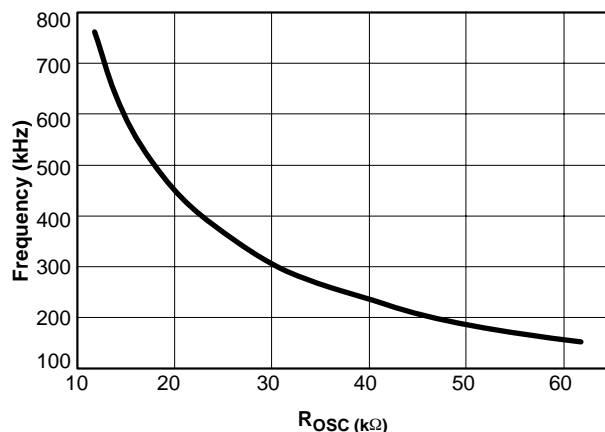
Figure 8. Switching Frequency
