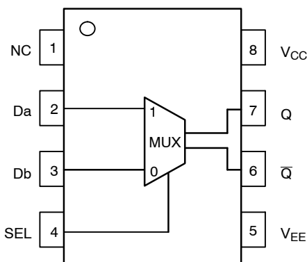
Figure 1. Logic Diagram and Pinout Assignment
