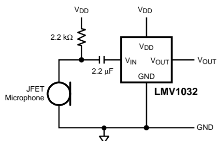
Figure 25. LMV1032 as External Pre-Amplifier
