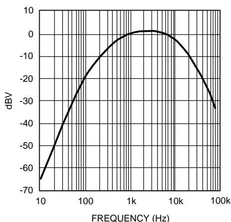
Figure 21. A-Weighted Filter
