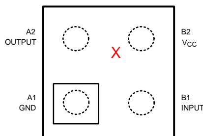
Figure 1. Top View
