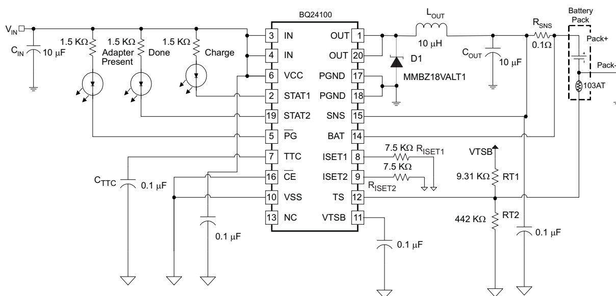
Figure 13. Stand-Alone, 1-Cell Application
