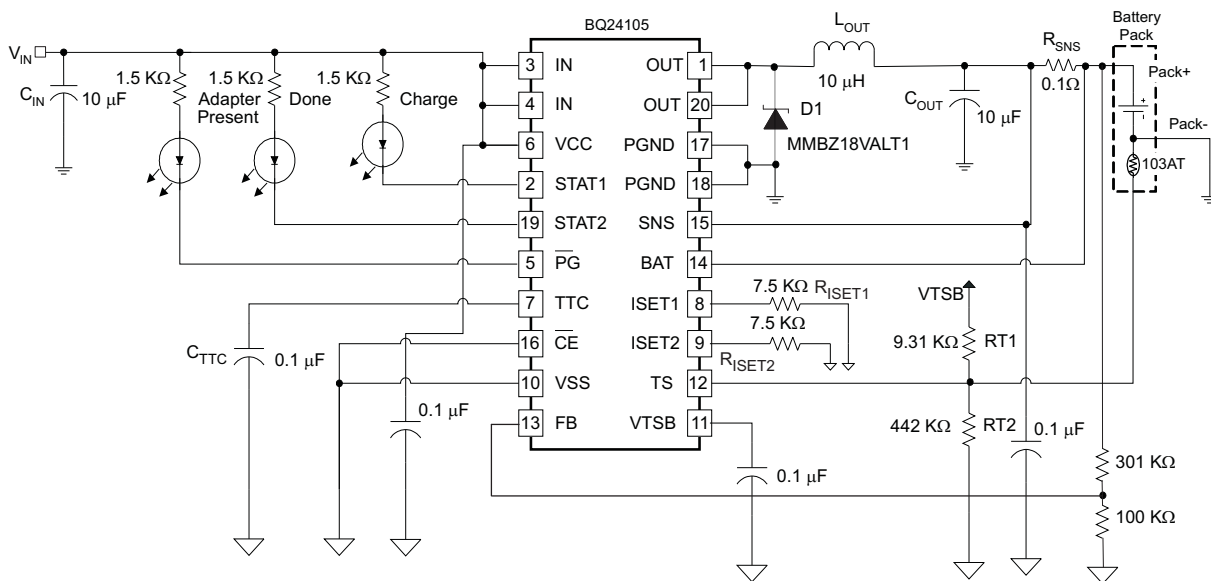
Figure 17. Stand-Alone, 2-Cell Application
