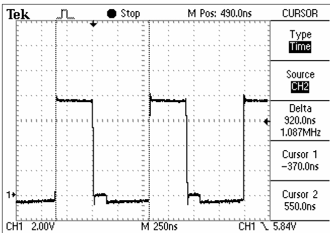
Figure 21. Precharge Waveform
