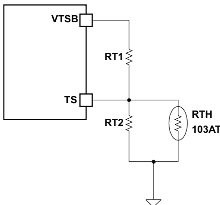
Figure 14. TS Resistor Network
