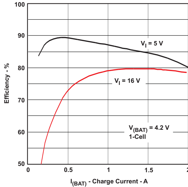
Figure 15. Efficiency vs Charge Current
