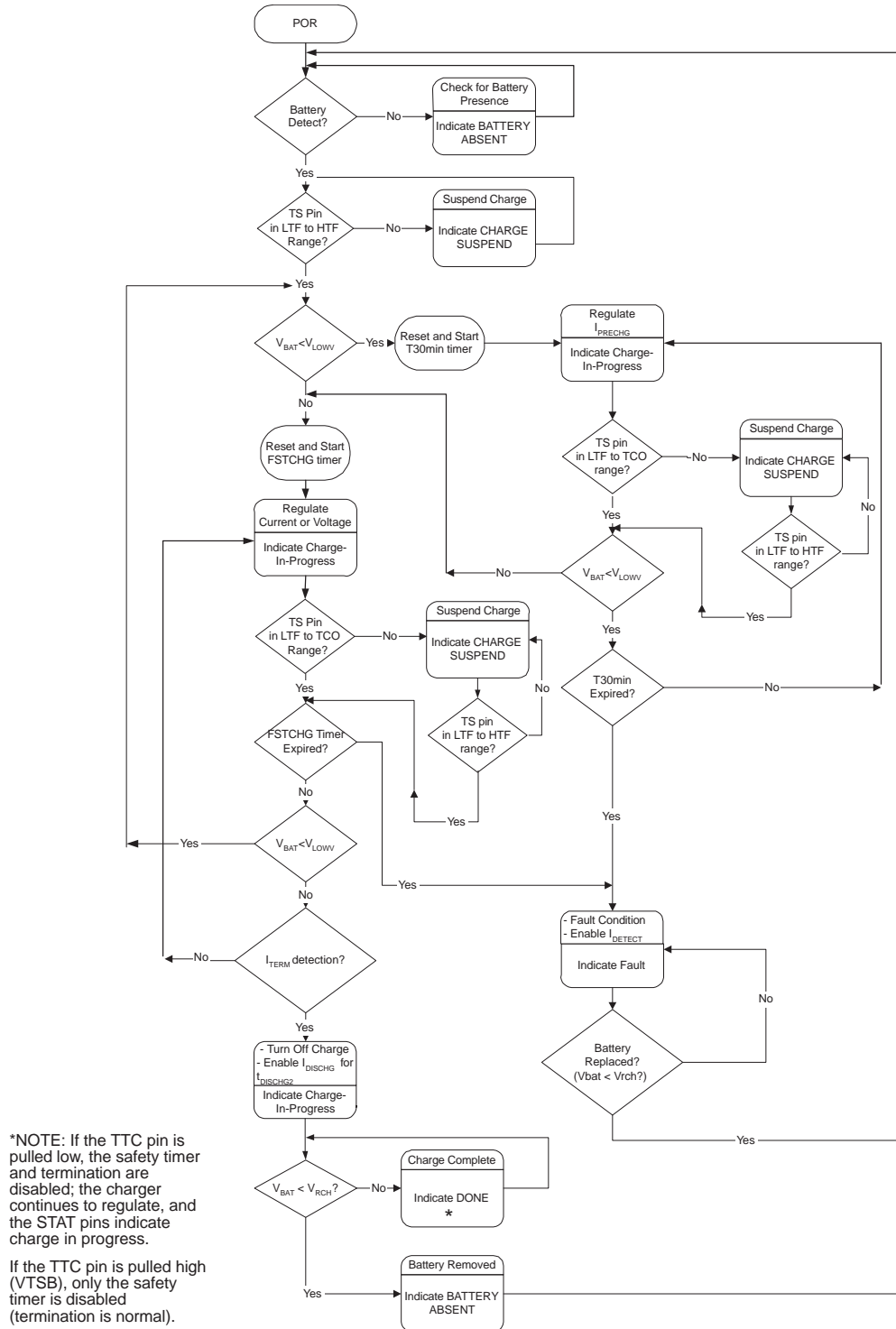
Figure 11. Stand-Alone Version Operational Flow Chart
