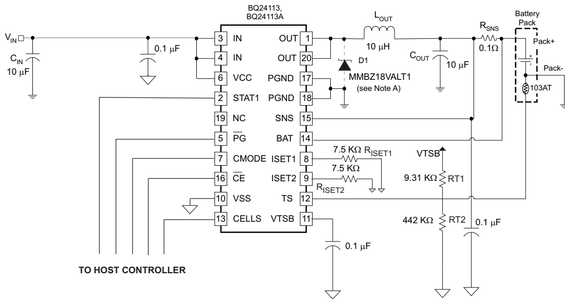
Figure 18. System-Controlled Application
