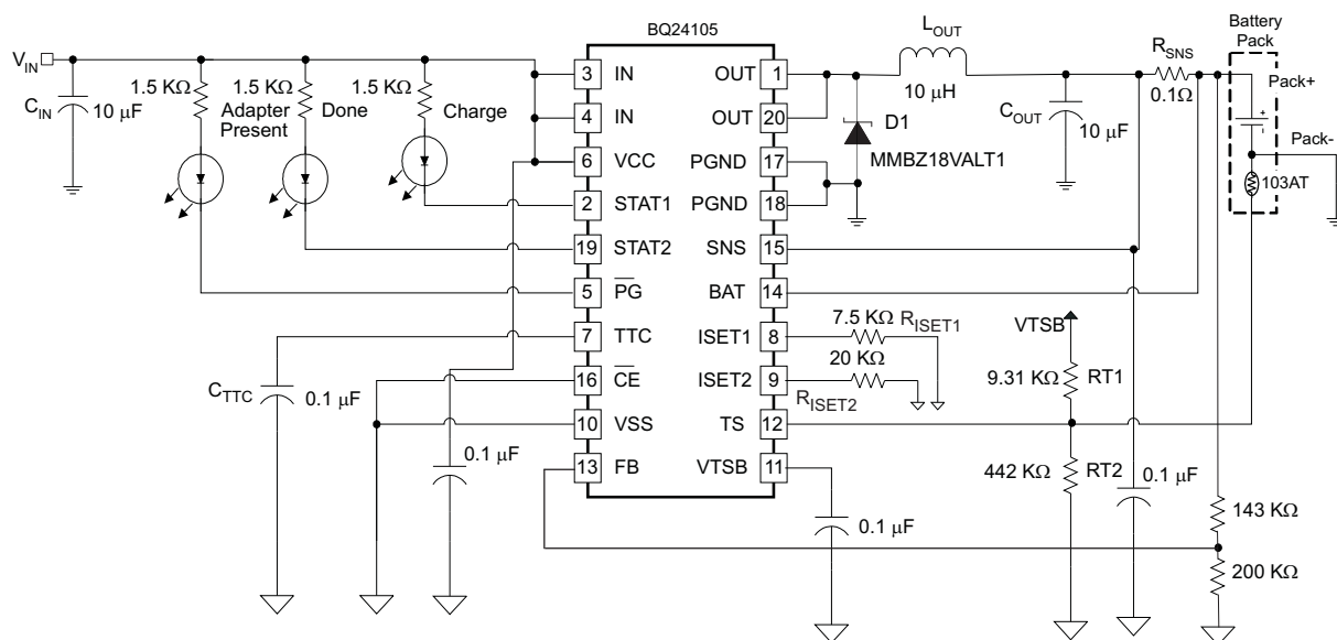
Figure 20. 1-Cell LiFePO4 Application
