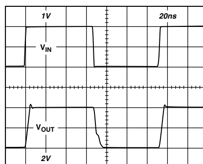
TPC 24. Large Signal Pulse Response, Gain = +2 ( R_{FB} = 750 \Omega , R_L = 150 \Omega , V_S = \pm 7.5 V )
