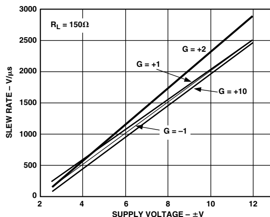
TPC 16. Maximum Slew Rate vs. Supply Voltage
