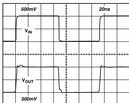
TPC 21. Small Signal Pulse Response, Gain = +1 ( R_{FB} = 5 k\Omega , R_L = 150 \Omega , V_S = \pm 7.5 V )
