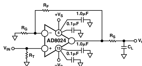
Figure 3. Circuit for Driving a Capacitive Load
