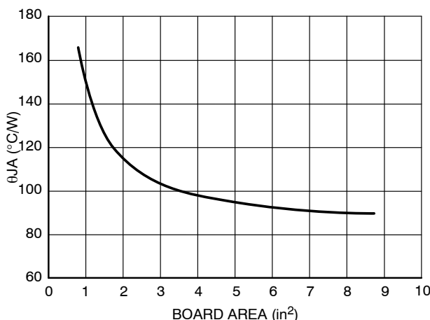
Figure 11. \theta_{JA} versus Board Area
