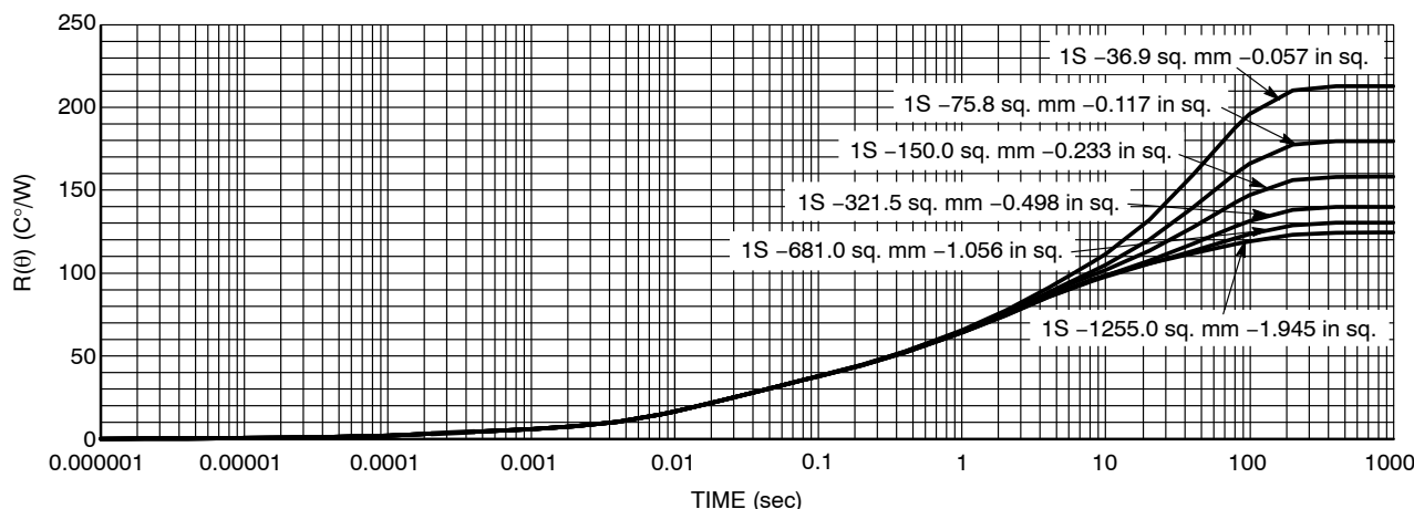
Figure 12. Transient Thermal Response
