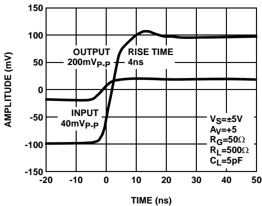
FIGURE 29. SMALL SIGNAL PULSE RESPONSE/RISE TIME
