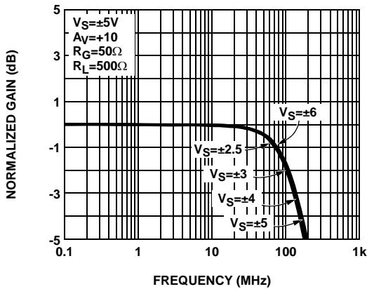
FIGURE 15. GAIN vs FREQUENCY FOR VARIOUS V_S ( A_V=+10 )
