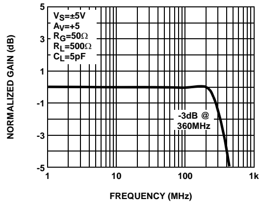
FIGURE 16. FREQUENCY RESPONSE (-3dB ROLL-OFF)
