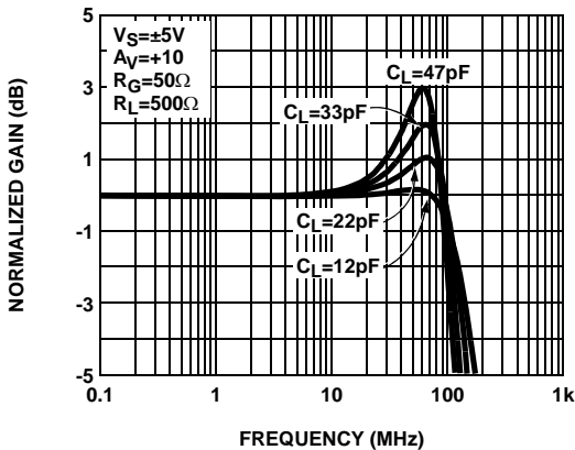
FIGURE 11. GAIN vs FREQUENCY FOR VARIOUS C_L ( A_V=+10 )
