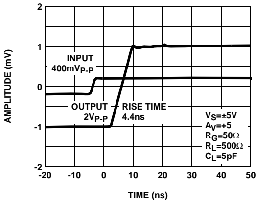
FIGURE 31. LARGE SIGNAL PULSE RESPONSE/RISE TIME
