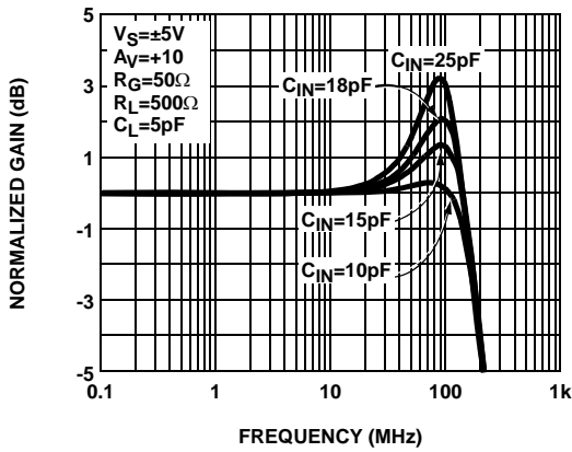
FIGURE 13. GAIN vs FREQUENCY FOR VARIOUS C_{IN} ( A_V=+10 )
