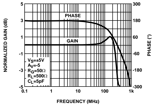
FIGURE 2. GAIN AND PHASE vs FREQUENCY (INVERTING)
