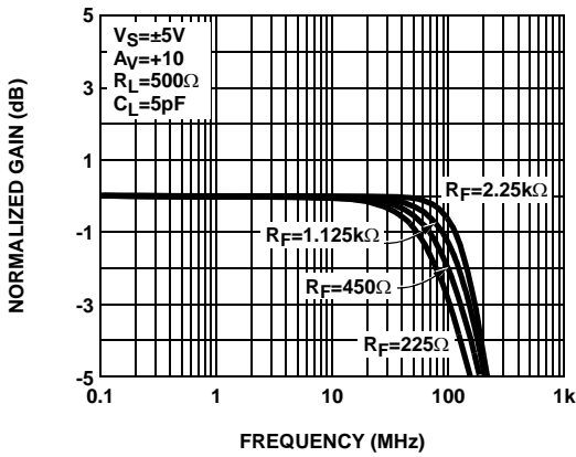
FIGURE 9. GAIN vs FREQUENCY FOR VARIOUS R_F ( A_V=+10 )
