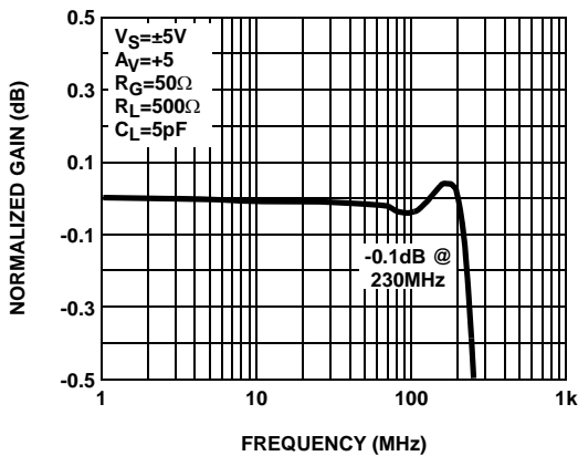
FIGURE 17. FREQUENCY RESPONSE (0.1dB GAIN FLATNESS)
