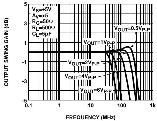
FIGURE 28. OUTPUT SWING vs FREQUENCY
