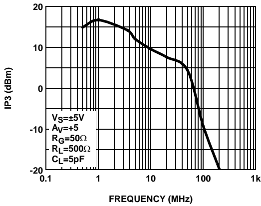
FIGURE 37. THIRD-ORDER INTERCEPT POINT
