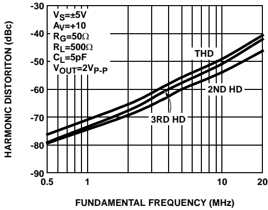
FIGURE 25. HARMONIC DISTORTION vs FREQUENCY (AV=+10)
