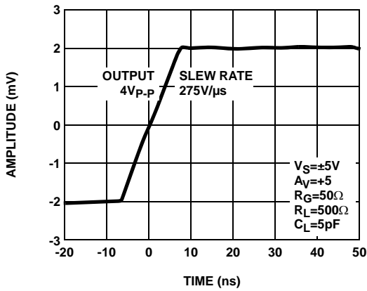
FIGURE 33. SLEW RATE (POSITIVE)
