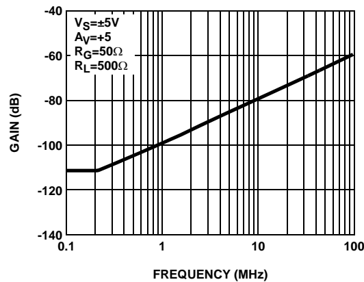
FIGURE 18. INPUT AND OUTPUT ISOLATION FOR DISABLE AMPLIFIER
