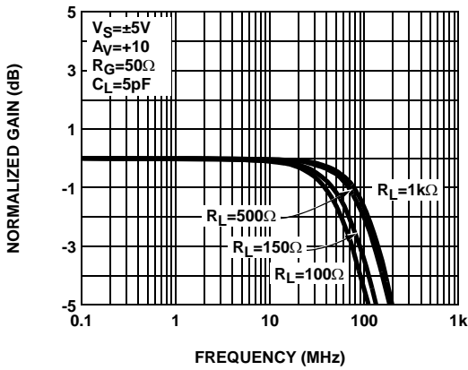
FIGURE 7. GAIN vs FREQUENCY FOR VARIOUS R_L ( A_V=+10 )
