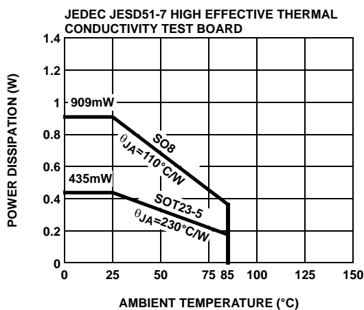
FIGURE 42. PACKAGE POWER DISSIPATION vs AMBIENT TEMPERATURE
