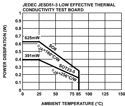
FIGURE 43. PACKAGE POWER DISSIPATION vs AMBIENT TEMPERATURE
