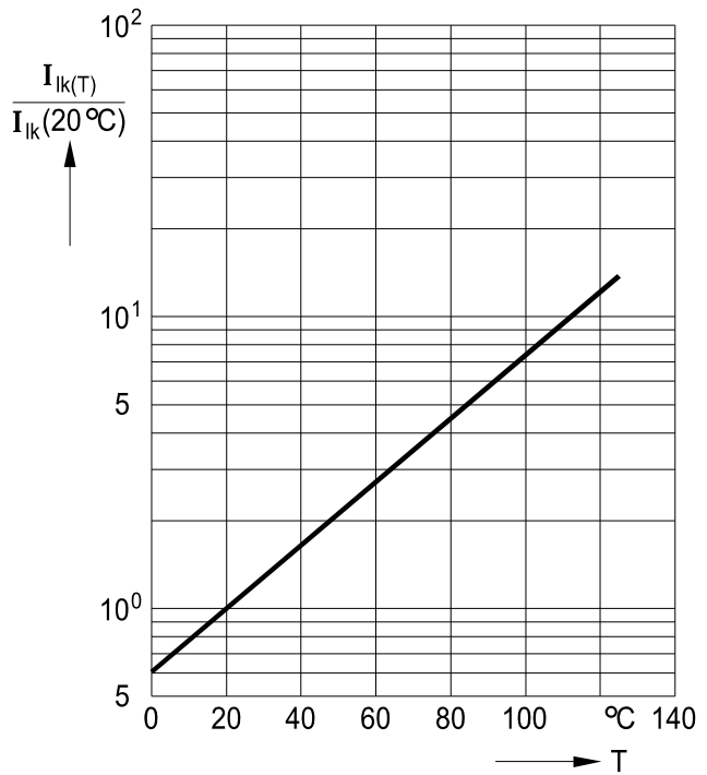
Leakage current versus temperature
