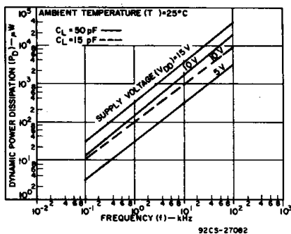
Fig. 7 – Typical dynamic power dissipation characteristics.
