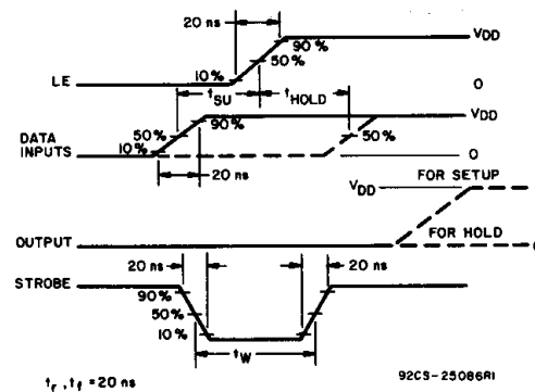
Fig. 14 - Dynamic waveforms.
