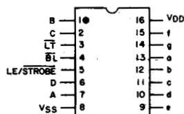
TOP VIEW 92CS-25084R1 CD4511B TERMINAL ASSIGNMENT
