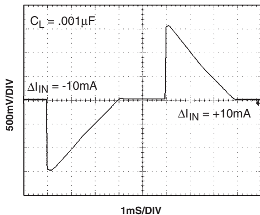
10mA LOAD TRANSIENT RESPONSE
