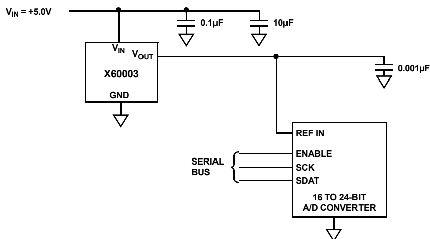
FIGURE 2. TYPICAL APPLICATION PRECISION 16 TO 24-BIT A/D CONVERTER
