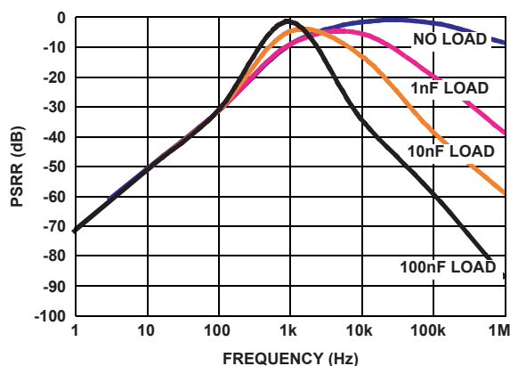
FIGURE 10. PSRR vs CAP LOAD
