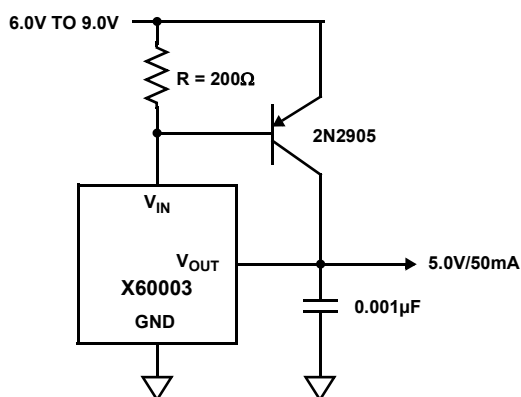
FIGURE 36. PRECISION 5V, 50mA REFERENCE
