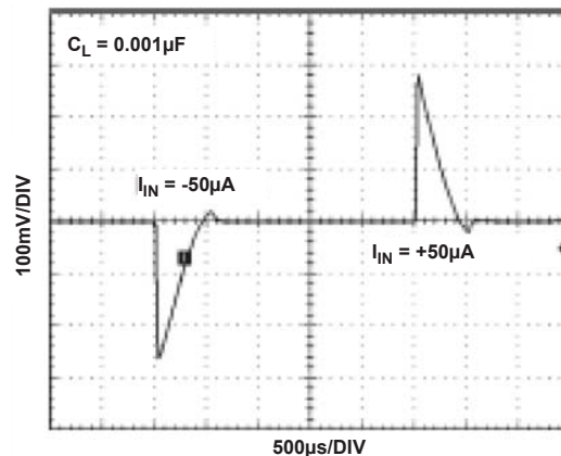
FIGURE 24. 50µA LOAD TRANSIENT RESPONSE
