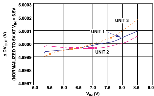
FIGURE 18. LINE REGULATION (3 UNITS)
