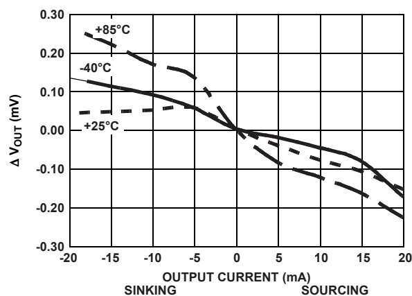
FIGURE 11. LOAD REGULATION
