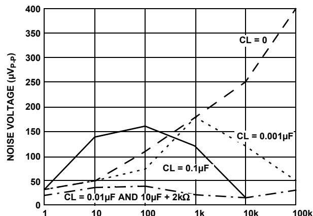
FIGURE 34. X60003 NOISE REDUCTION
