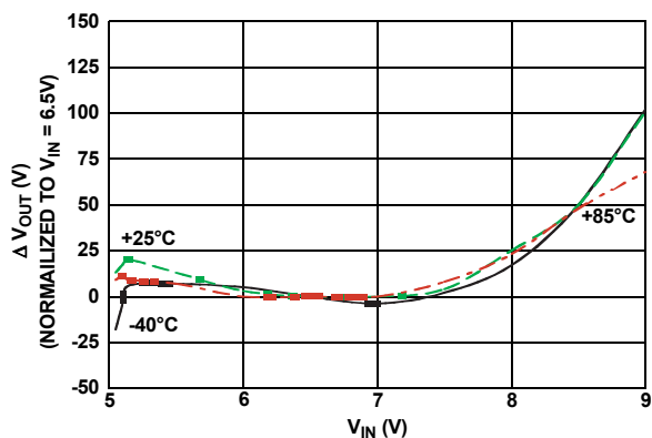
FIGURE 17. LINE REGULATION
