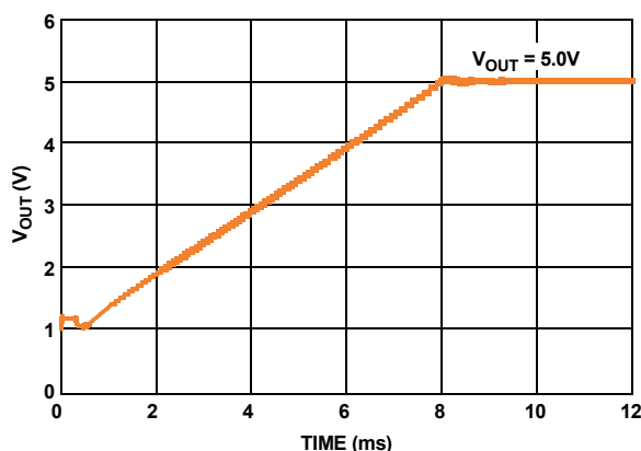
FIGURE 31. TURN-ON TIME
