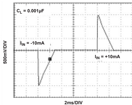
FIGURE 23. 10mA LOAD TRANSIENT RESPONSE
