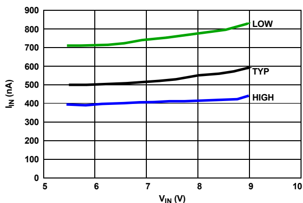
FIGURE 30. I_{IN} vs V_{IN} (3 UNITS)
