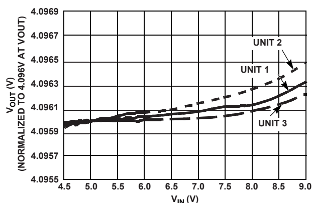
FIGURE 6. LINE REGULATION (3 UNITS)
