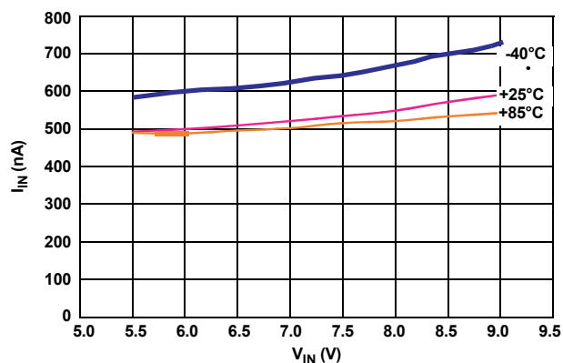
FIGURE 29. I_{IN} vs V_{IN}
