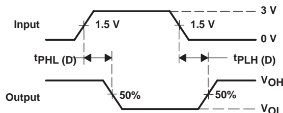
VOLTAGE WAVEFORMS
