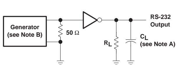
TEST CIRCUIT
