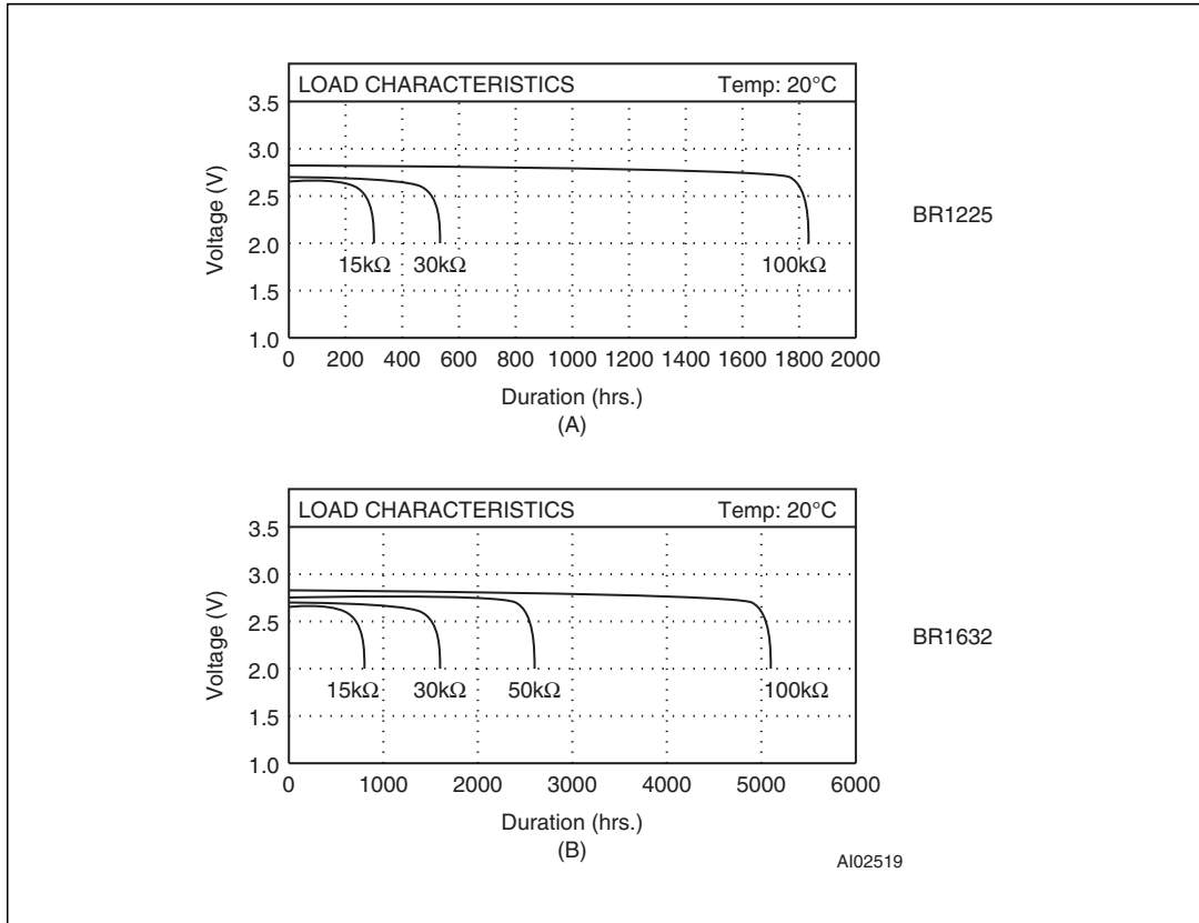
Figure 3. Battery discharge rates
