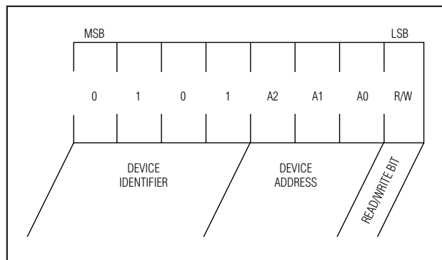
Figure 3. Control Byte
