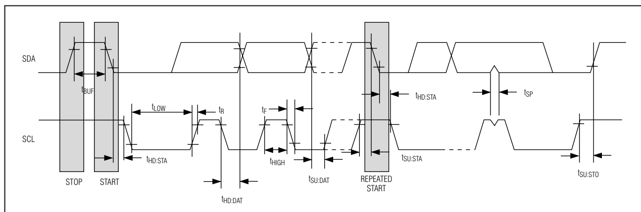
Figure 6. Timing Diagram
