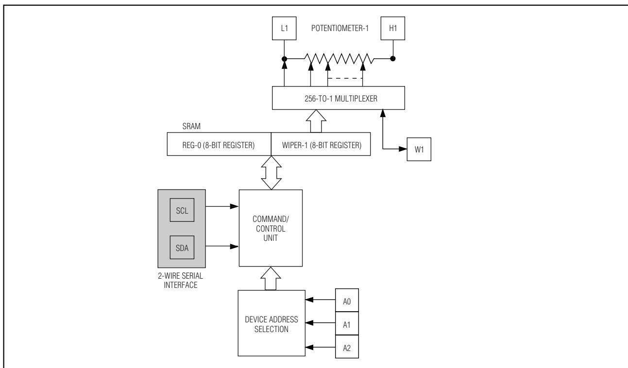
Figure 1. Functional Diagram
