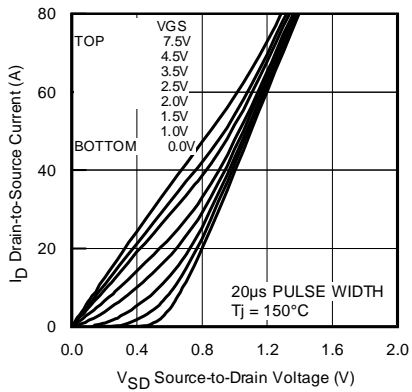
Fig. 9. Typical Reverse Output Characteristics
