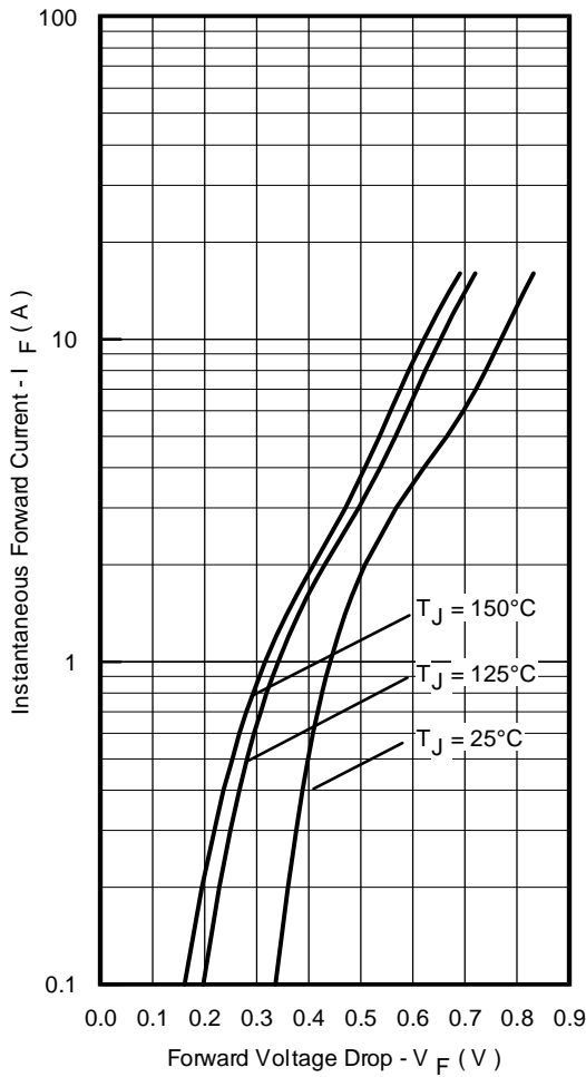
Fig. 29 - Maximum Forward Voltage Drop Characteristics
