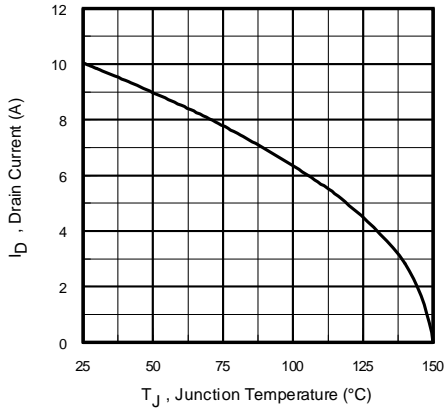
Fig 25. Maximum Drain Current Vs. Case Temperature
