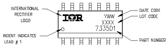
TOP MARKING
