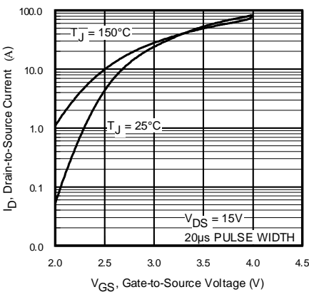
Fig 5. Typical Transfer Characteristics
