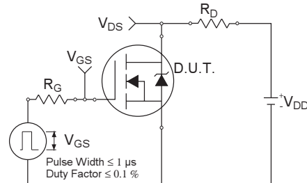
Fig 26a. Switching Time Test Circuit
