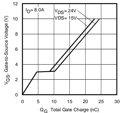
Fig 16. Gate-to-Source Voltage vs Typical Gate Charge
