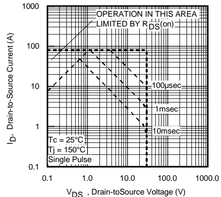
Fig 18. Maximum Safe Operating Area
