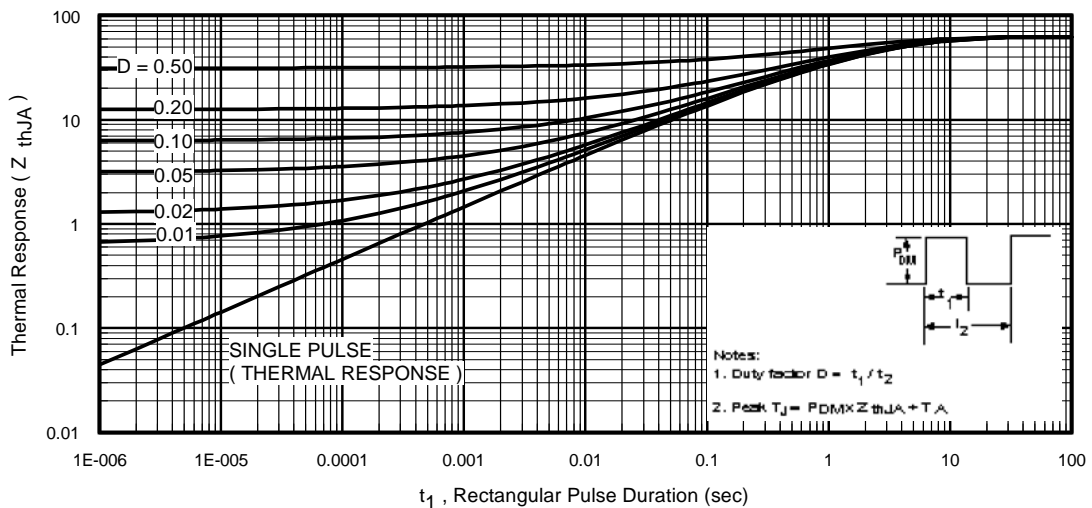
Fig. 28. Maximum Effective Transient Thermal Impedance, Junction-to-Ambient
