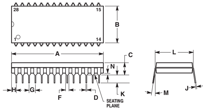
Figure 20. Plastic 28-Pin DIP (Case 710)
