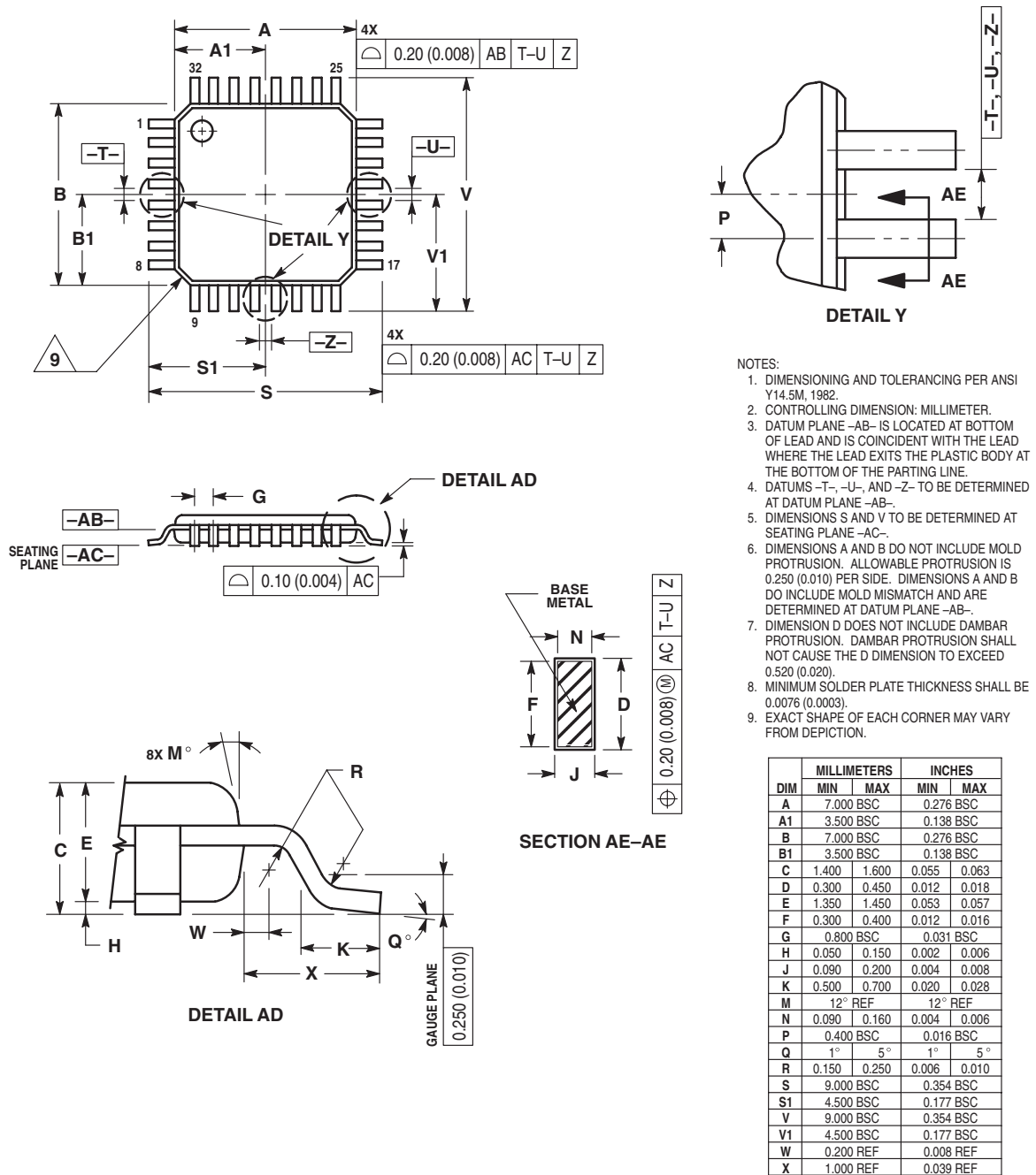
Figure 22. Plastic 32-Pin QFP (Case 873A)
