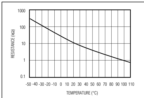
Figure 9. Typical Thermistor Characteristics
