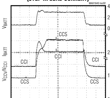
LOAD-TRANSIENT RESPONSE (STEP IN LOAD CURRENT)
