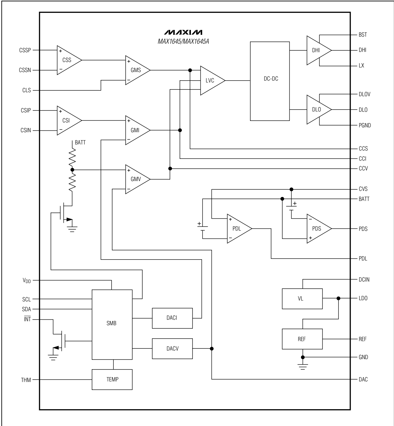
Figure 2. Functional Diagram
