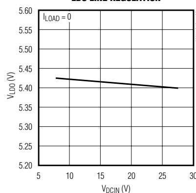
LDO LINE REGULATION
