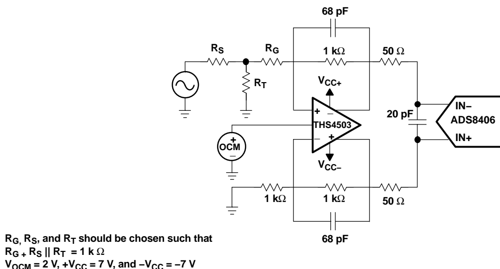
Figure 33. Using the THS4503 With the ADS8406
