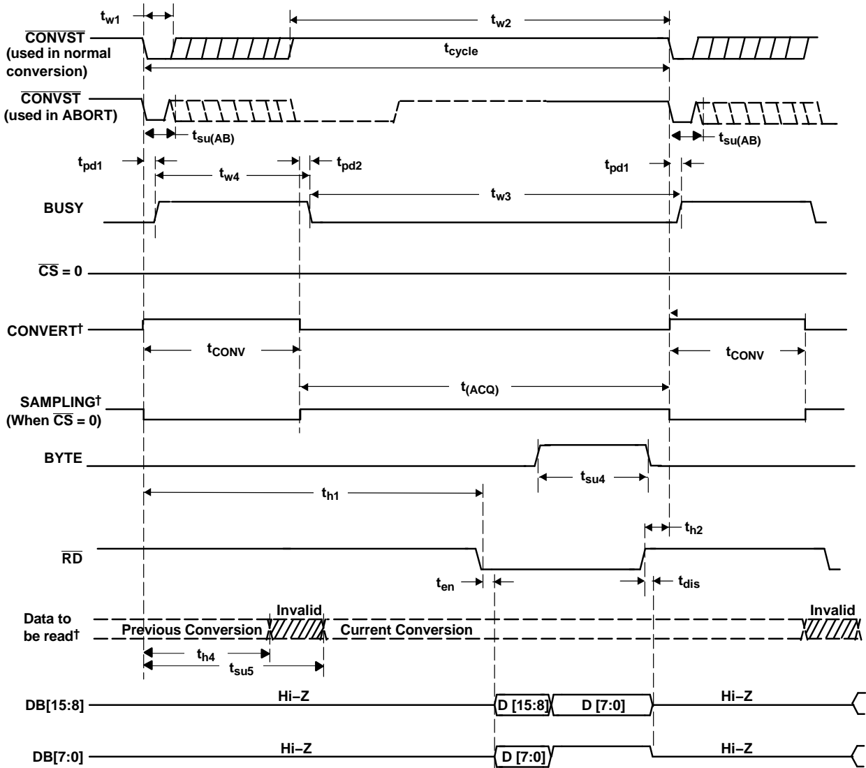
Figure 3. Timing for Conversion and Acquisition Cycles With \overline{\text{CS}} Tied to \text{BDGND} , \overline{\text{RD}} Toggling
