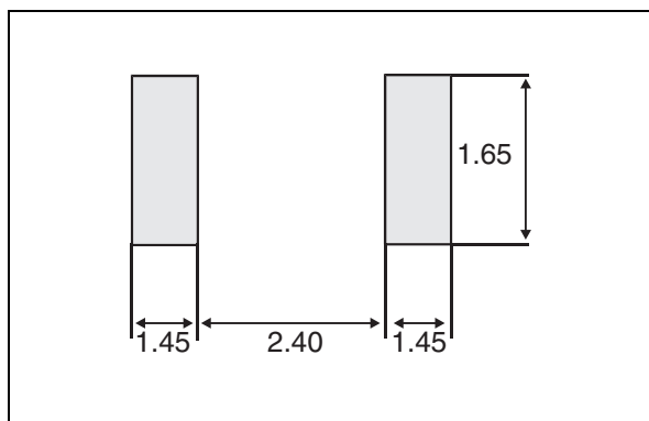
Figure 15: SMA Foot Print Dimensions
