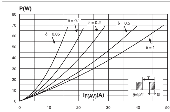
Figure 1. Conduction losses versus average current (per diode)
