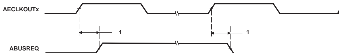
Figure 7–21. BUSREQ Timing for EMIFA
