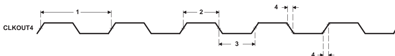
Figure 7–2. CLKOUT4 Timing
