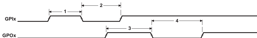
Figure 7–45. GPIO Port Timing
