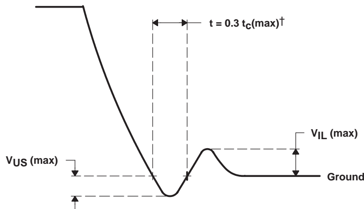
Figure 6–5. AC Transient Specification Fall Time
