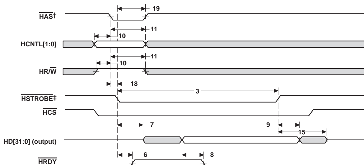
Figure 7–35. HPI32 Read Timing ( \overline{\text{HAS}} Used)
