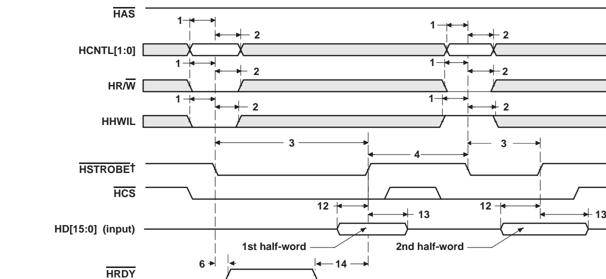
Figure 7-32. HPI16 Write Timing ( \overline{\text{HAS}} Not Used, Tied High)
