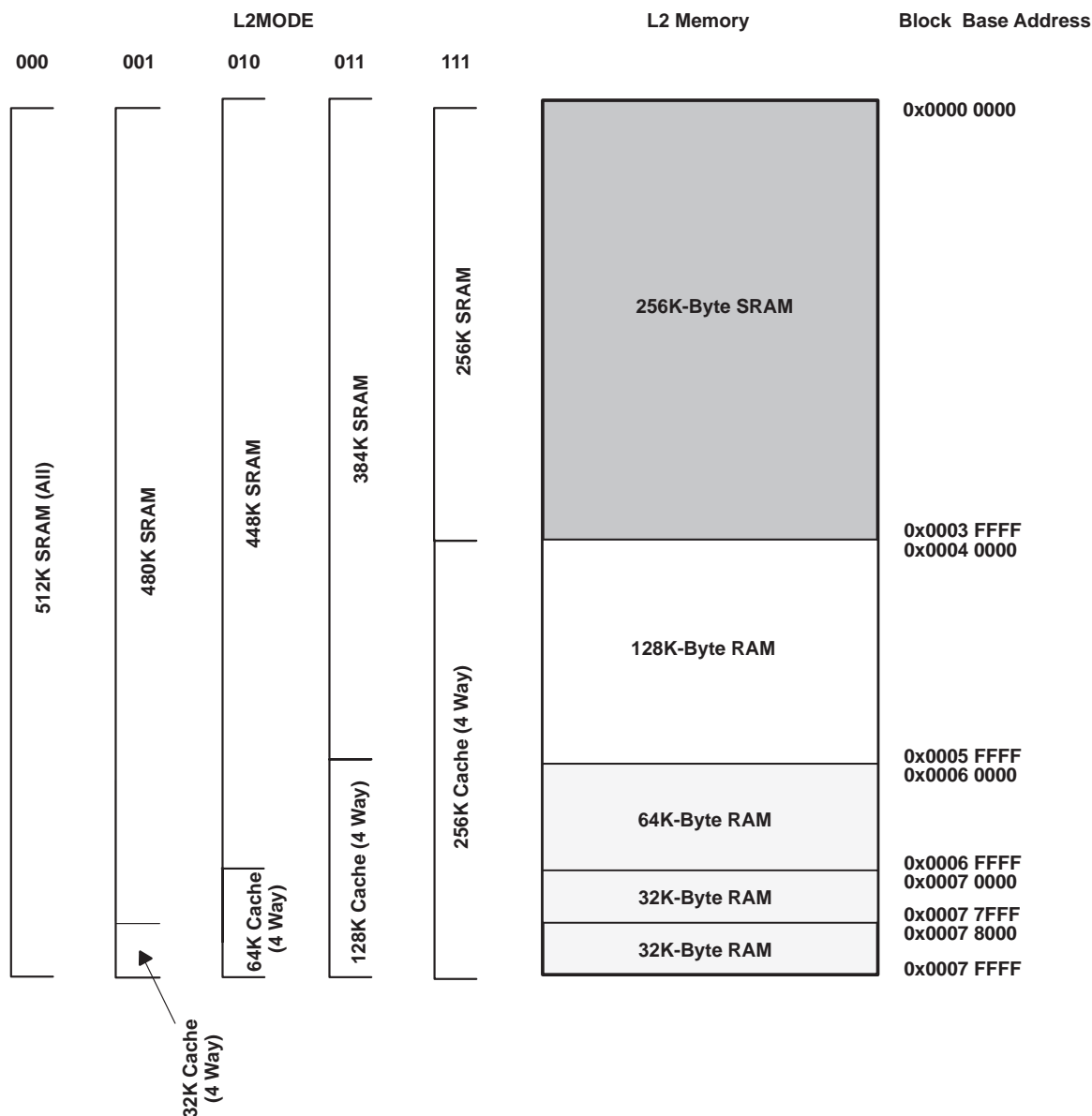
Figure 2–4. TMS320C6418 L2 Architecture Memory Configuration
