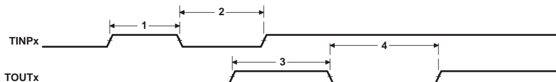
Figure 7–44. Timer Timing
