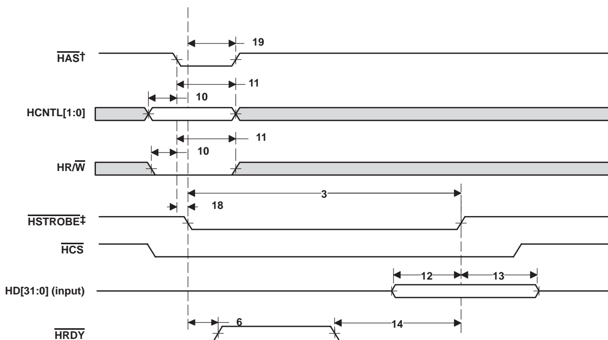
Figure 7–37. HPI32 Write Timing ( \overline{\text{HAS}} Used)
