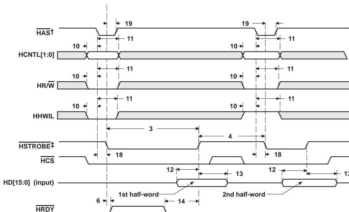
Figure 7-33. HPI16 Write Timing ( \overline{\text{HAS}} Used)
