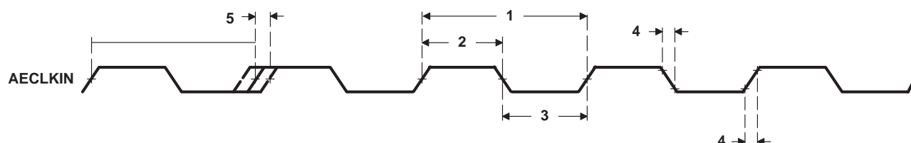
Figure 7–4. AECLKIN Timing for EMIFA
