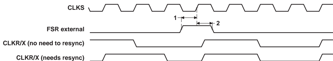
Figure 7–39. FSR Timing When GSYNC = 1
