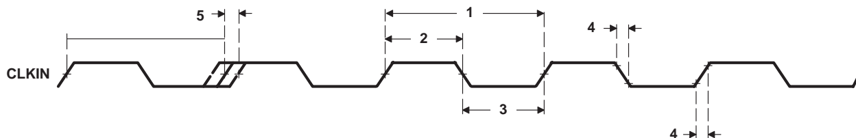
Figure 7–1. CLKIN Timing
