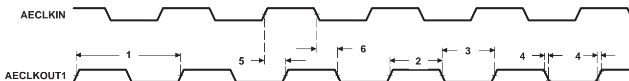
Figure 7–5. AECLKOUT1 Timing for the EMIFA Module
