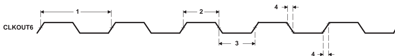
Figure 7–3. CLKOUT6 Timing
