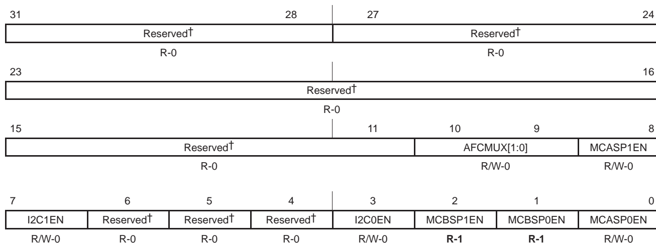
Figure 3–1. Peripheral Configuration Register (PERCFG) [Address Location: 0x01B3F000]
