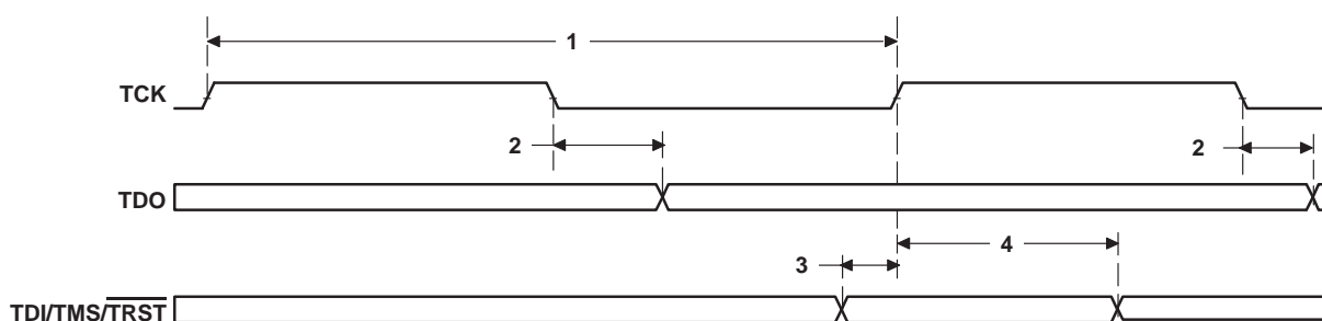
Figure 7–46. JTAG Test-Port Timing
