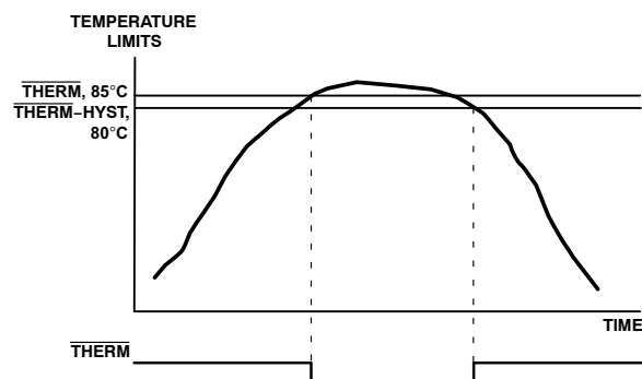
Figure 32. THERM Behavior
