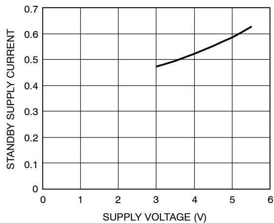
Figure 12. Standby Supply Current vs. Supply Voltage
