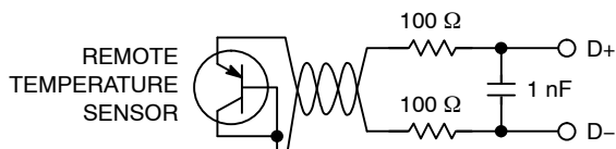
Figure 29. Filter between Remote Sensor and ADM1034
