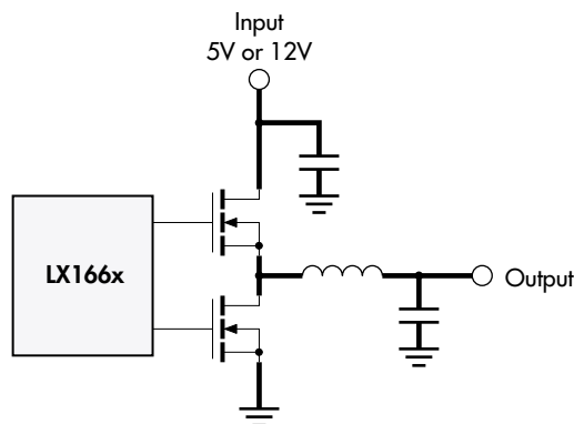
FIGURE 13 — Power Traces
