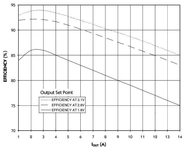
FIGURE 2 — Efficiency Test Results: Non-Synchronous Operation, V_{IN} = 5V
