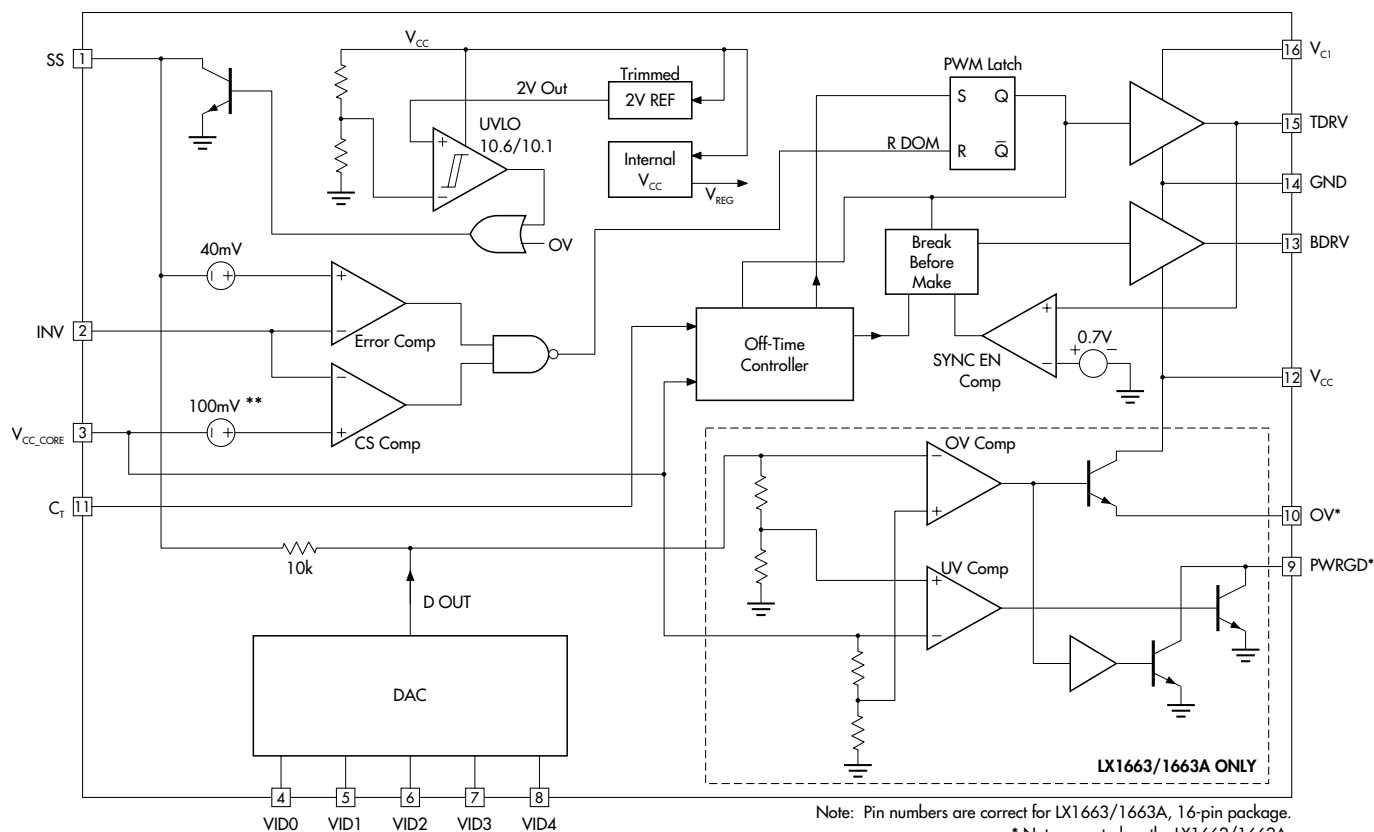
FIGURE 5 — Block Diagram
