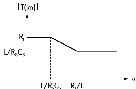
FIGURE 12 — Sensor Gain
