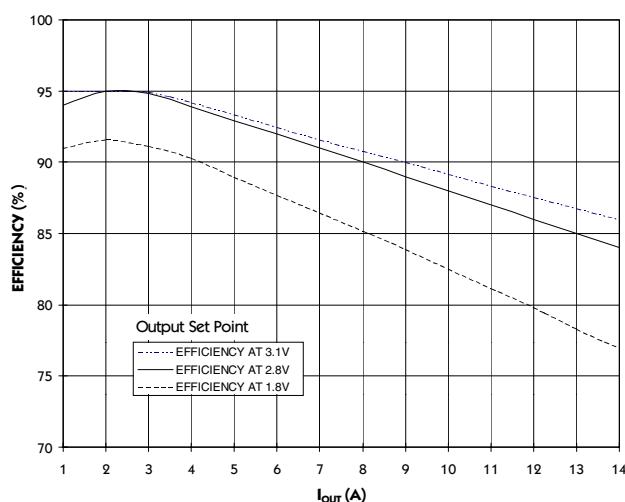
FIGURE 3 — Efficiency Test Results: Synchronous Operation, V_{IN} = 5V
