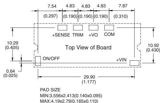
Figure 5. Recommended VPOL16A-12-SMT Footprint
