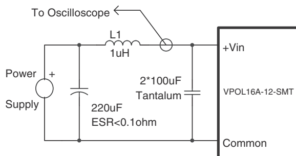
Figure 10. Input Reflected-Ripple Test Setup
