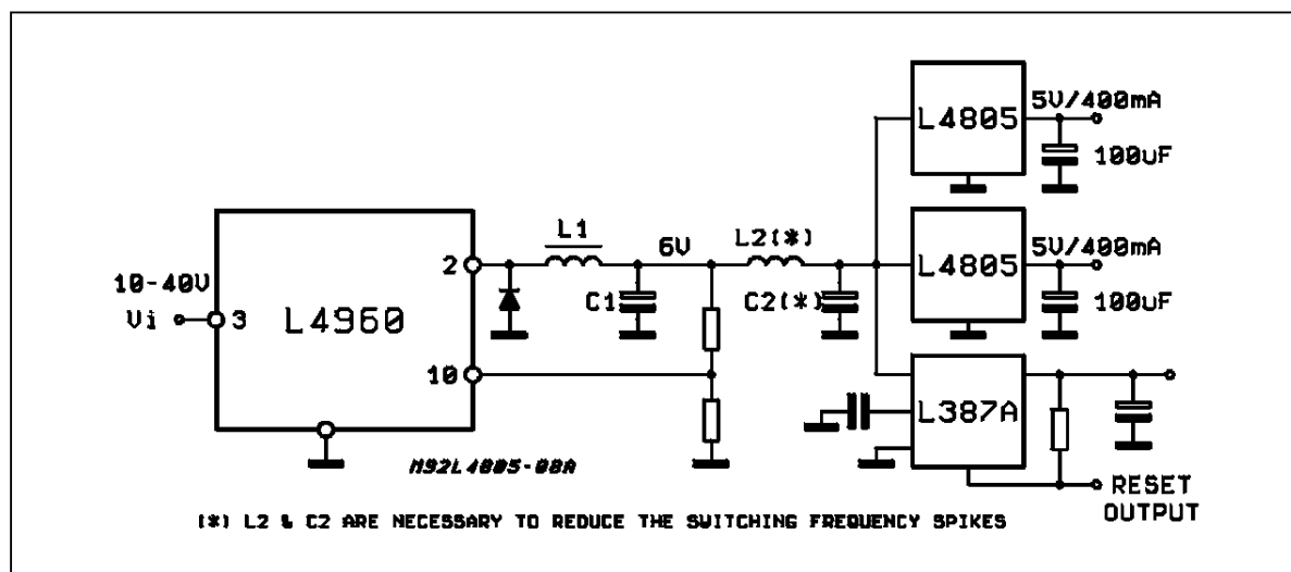
Figure 5: Preregulator for Distributed Supplies
