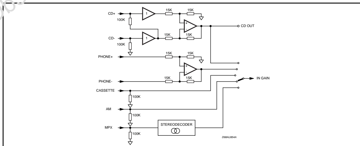
Figure 4. Input stages
