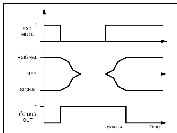
Figure 5. Softmute Timing
