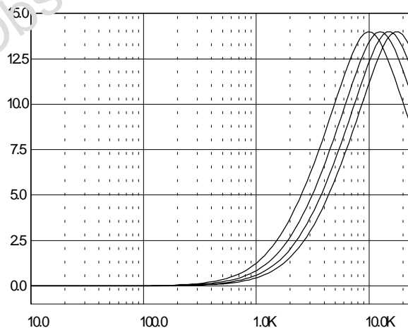
Figure 11. Treble Center Frequencies @ Gain = 14dB
