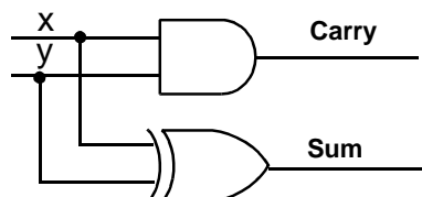
Figure 4. One-Bit Half Adder
