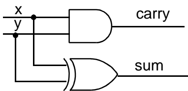
Figure 2. One-Bit Half Adder
