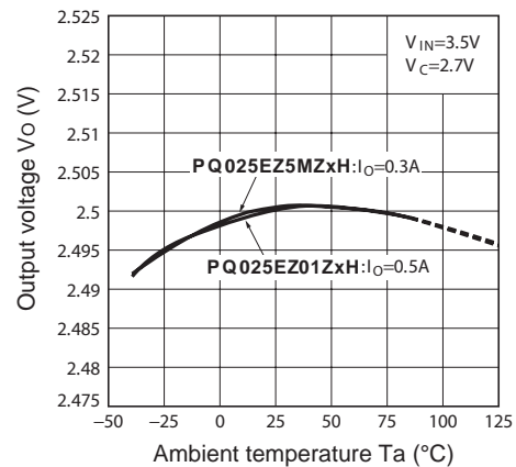
Fig.16 Output Voltage vs. Ambient Temperature (PQ025EZ5MZxH / PQ025EZ01ZxH)
