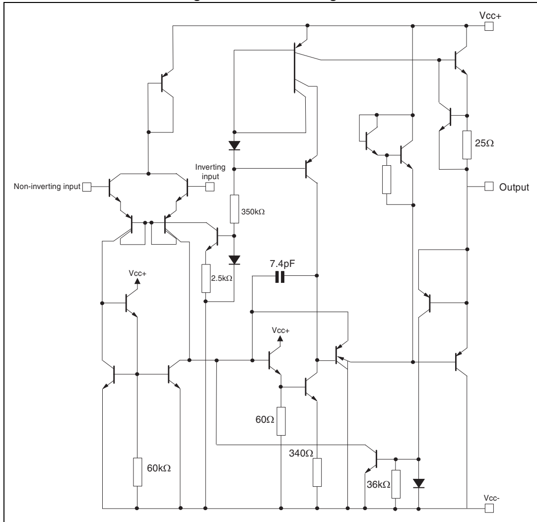
Figure 1. Schematic diagram
