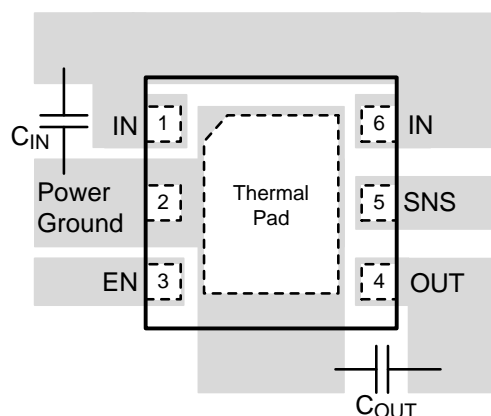
Figure 38. LP38692 WSON Package
