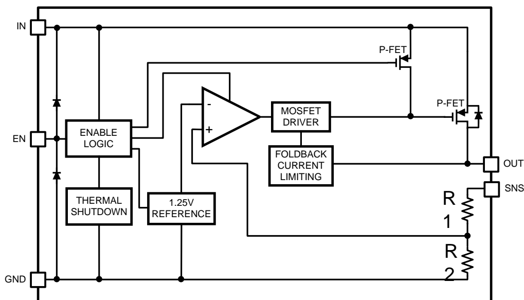
Figure 29. LP38692 Functional Diagram (WSO)
