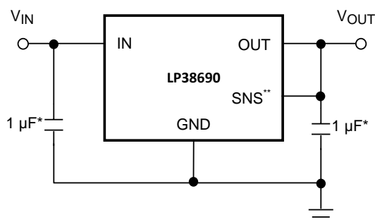
Figure 30. LP38690 Typical Application
