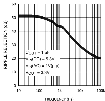
Figure 6. Ripple Rejection
