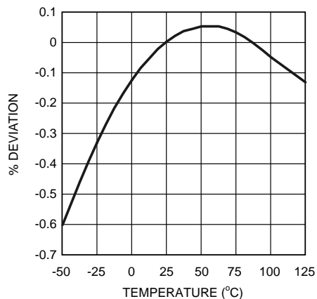
Figure 17. V_{OUT} vs Temperature (2.5 V)
