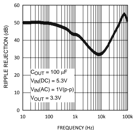
Figure 5. Ripple Rejection
