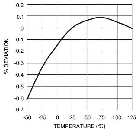
Figure 18. V_{OUT} vs Temperature (1.8 V)
