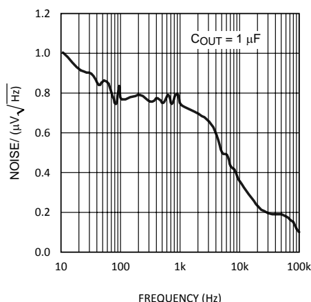
Figure 1. Noise vs Frequency
