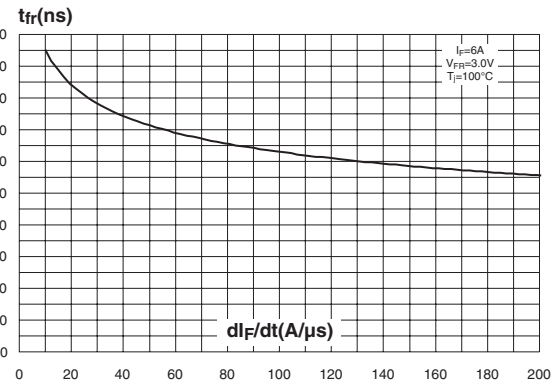
Figure 6: Forward recovery time versus di_F/dt (typical values)
