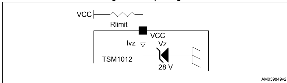
Figure 5. Clamp voltage
