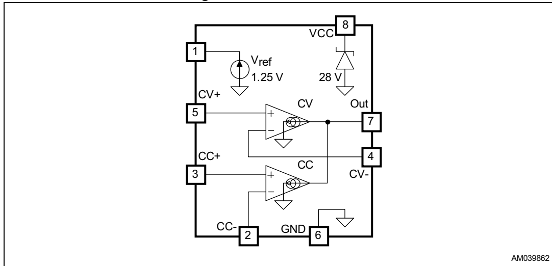
Figure 2. Internal schematic
