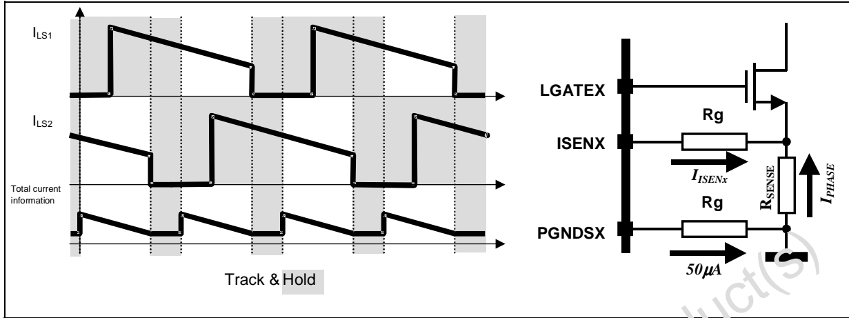
Figure 4. Current Reading Timing (Left) and Circuit (Right)
