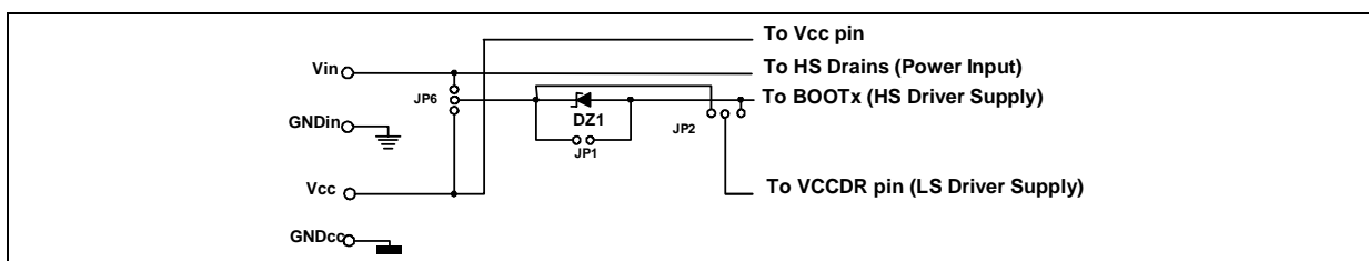
Figure 20. Power supply configuration
