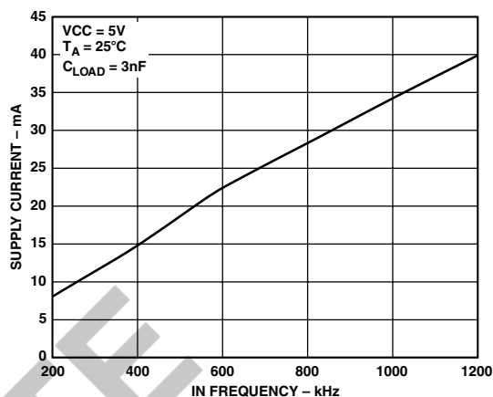
TPC 10. Supply Current vs. Frequency
