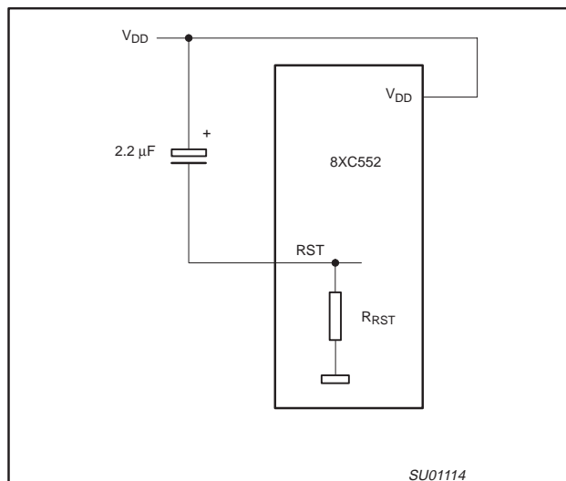
Figure 2. Power-On Reset
