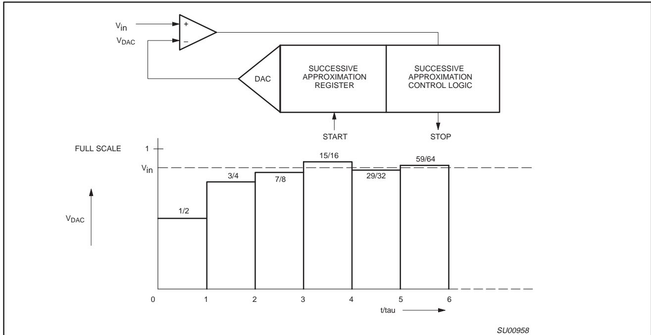
Figure 20. Successive Approximation ADC
