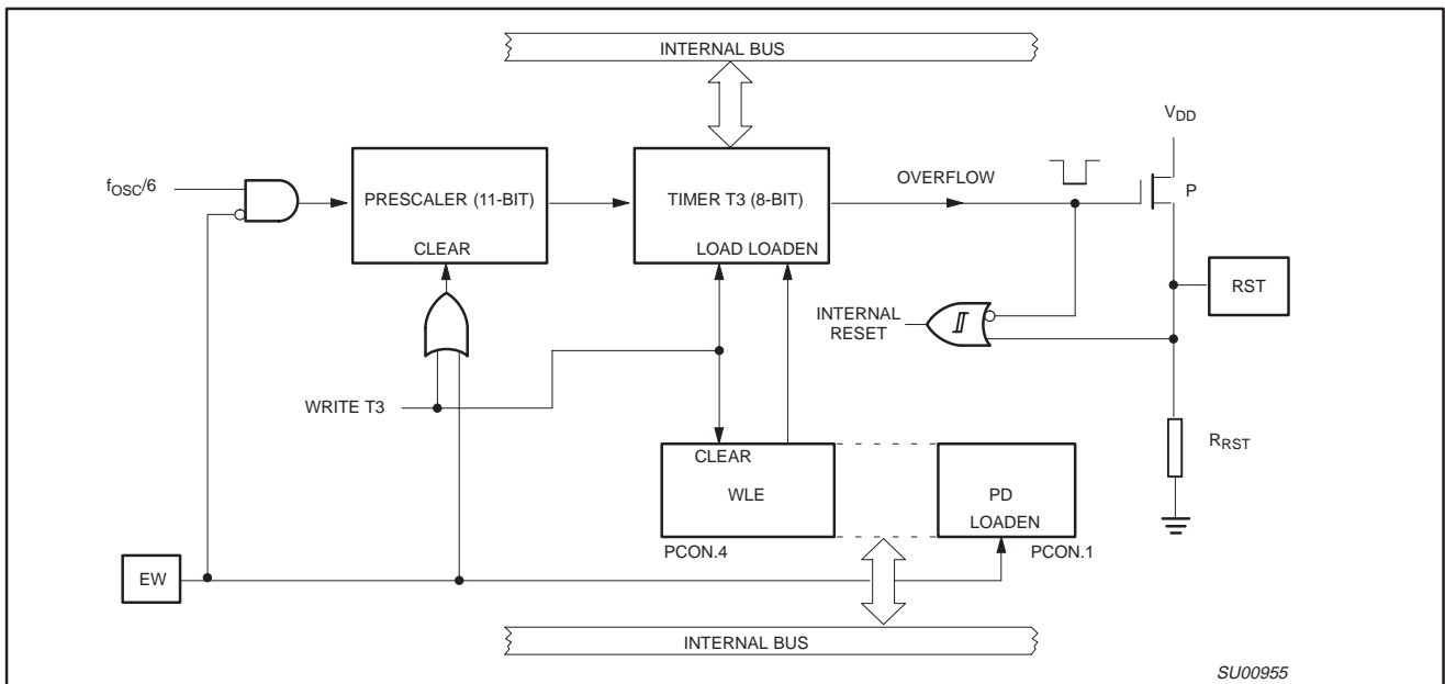
Figure 17. Watchdog Timer
