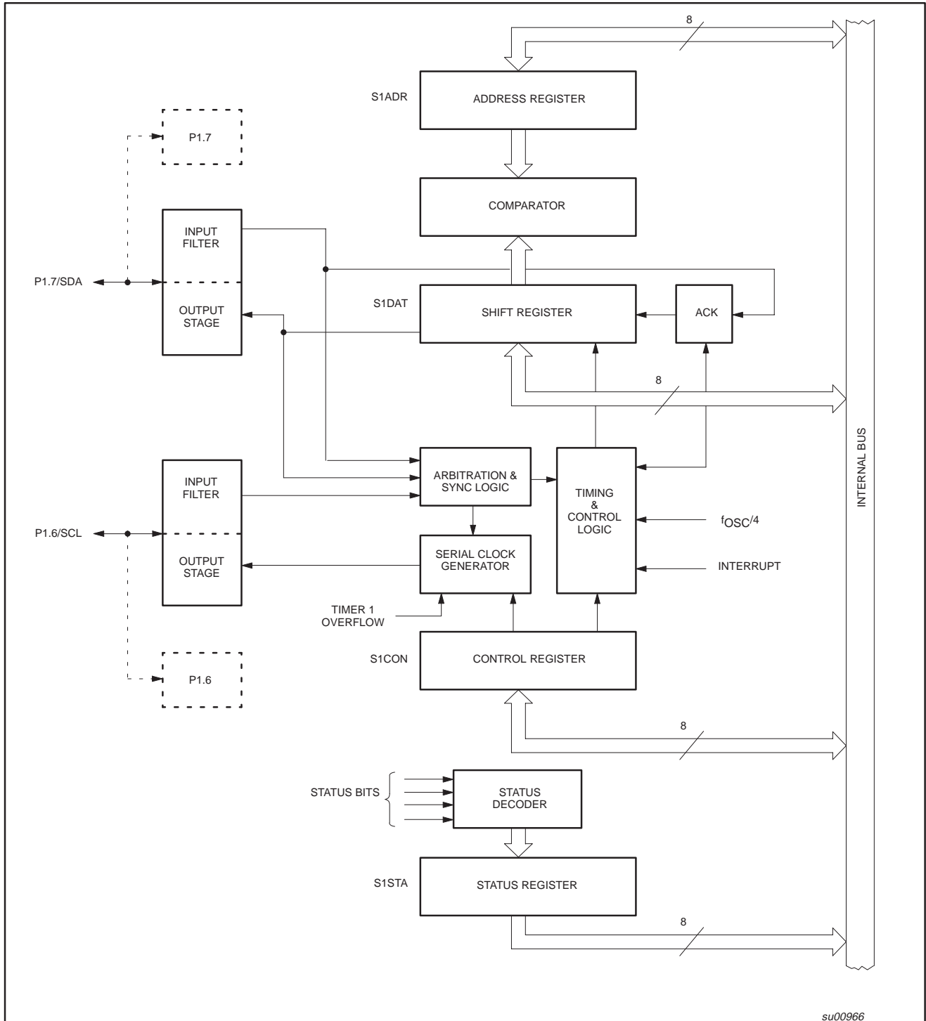
Figure 34. I 2 C Bus Serial Interface Block Diagram
