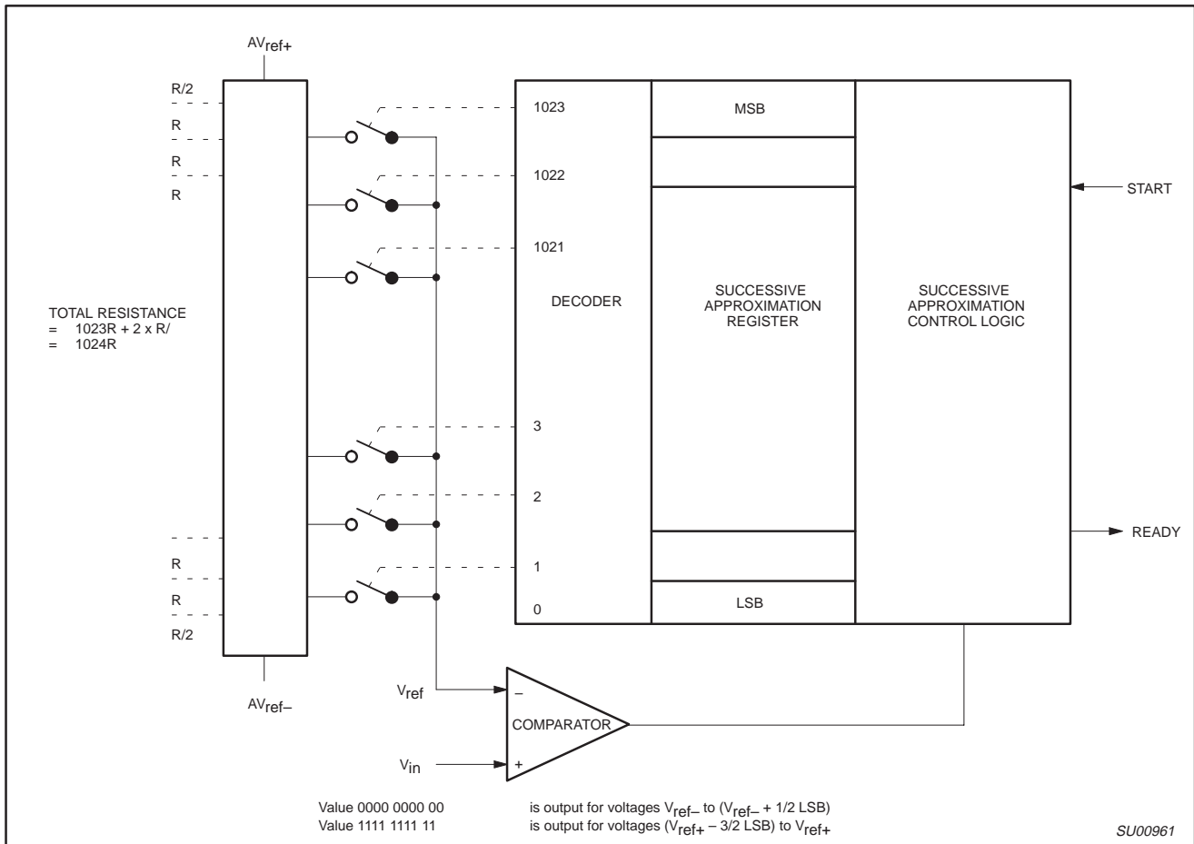
Figure 23. ADC Realization
