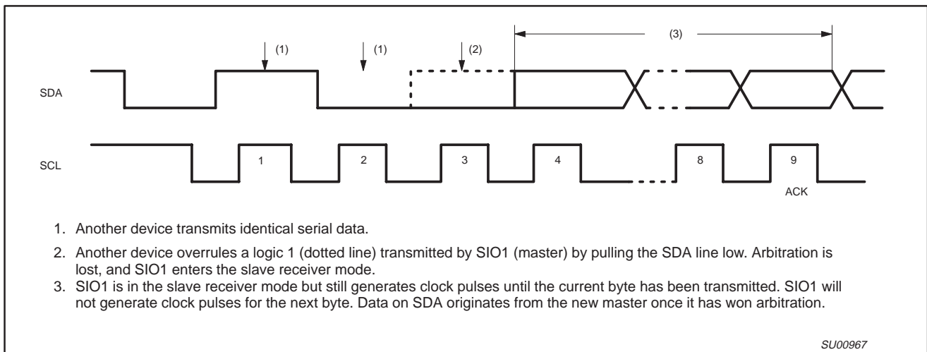
Figure 35. Arbitration Procedure
