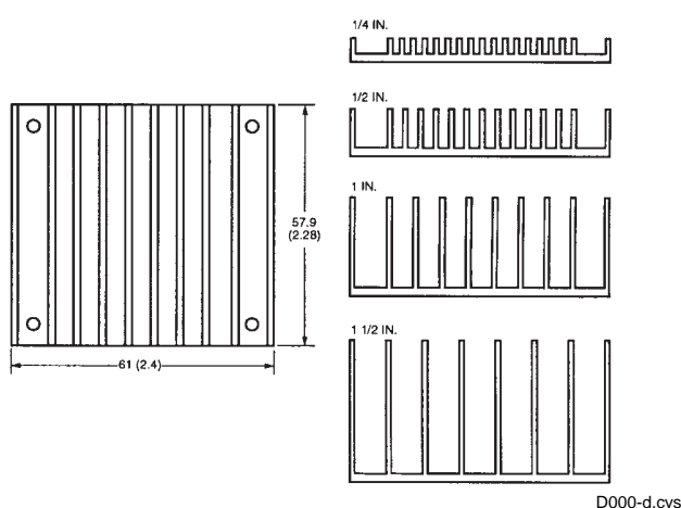
Figure 23. Transverse Heat Sink
