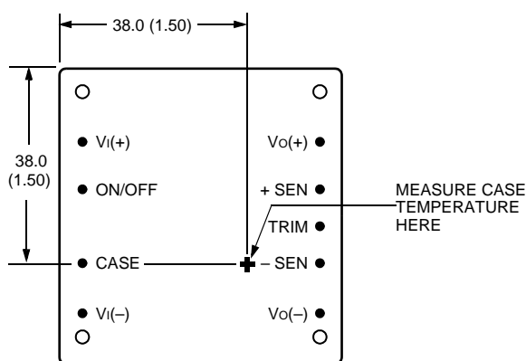
Figure 17. Case Temperature Measurement Location
