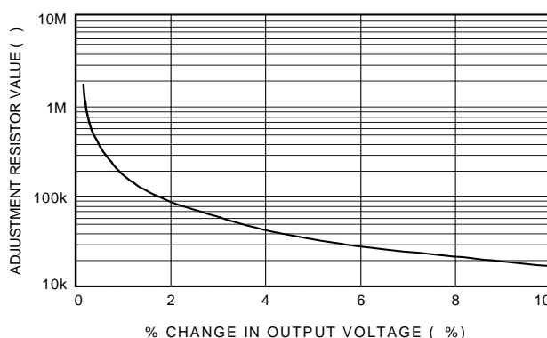
Figure 16. Resistor Selection for Increased Output Voltage
