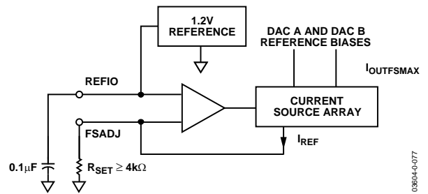
Figure 51. Reference Circuitry
