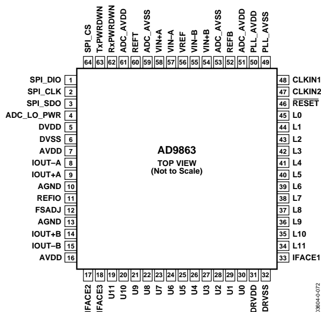
Figure 3. Pin Configuration
