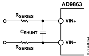
Figure 47. Typical Input
