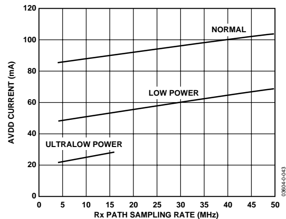
Figure 49. Typical Rx Path Analog Supply Current vs. Sample Rate, V_{DD} = 3.3 V for Normal, Low, and Ultralow Power Modes
