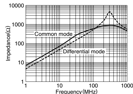
ACM1211-102-2PL-TL01
