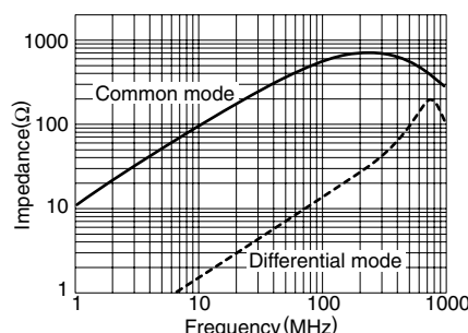
ACM4532-601-2P
