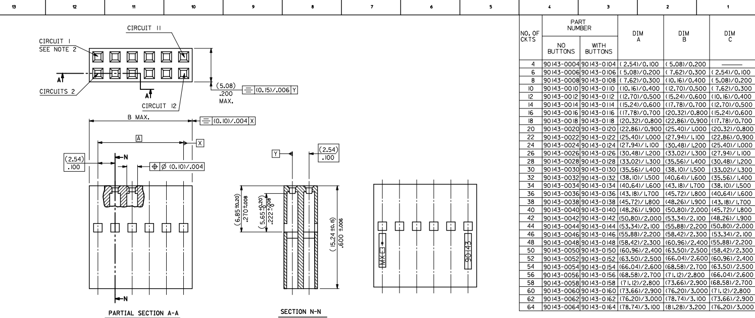
NO POLARISING BUTTON VERSION (90143-00** VERSION)
