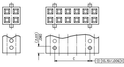
POLARISING BUTTON VERSION (90143-10** VERSION)
