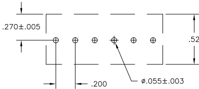
RECOMMENDED BOARD LAYOUT
