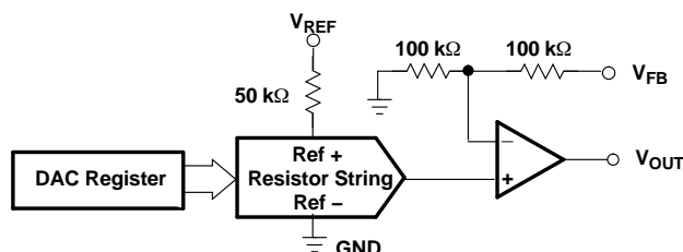
Figure 43. Typical DAC Architecture
