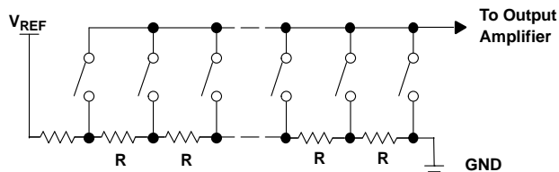
Figure 44. Typical Resistor String
