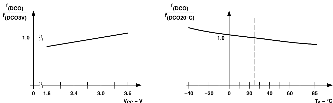
Figure 9. DCO Frequency vs Supply Voltage V CC and vs Ambient Temperature
