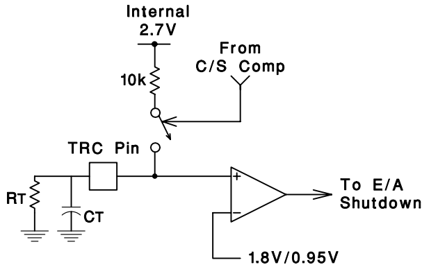
Figure 3. Timer Function
