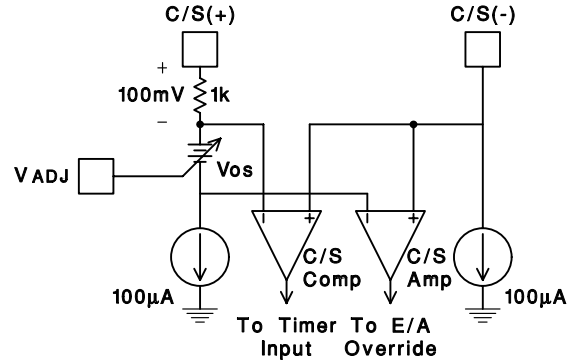
Figure 4. Current Sense Input Configuration
