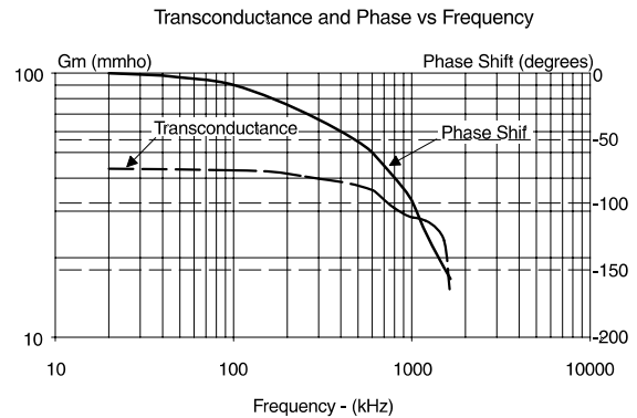
Figure 9. UCx832 Current Sense Amplifier
